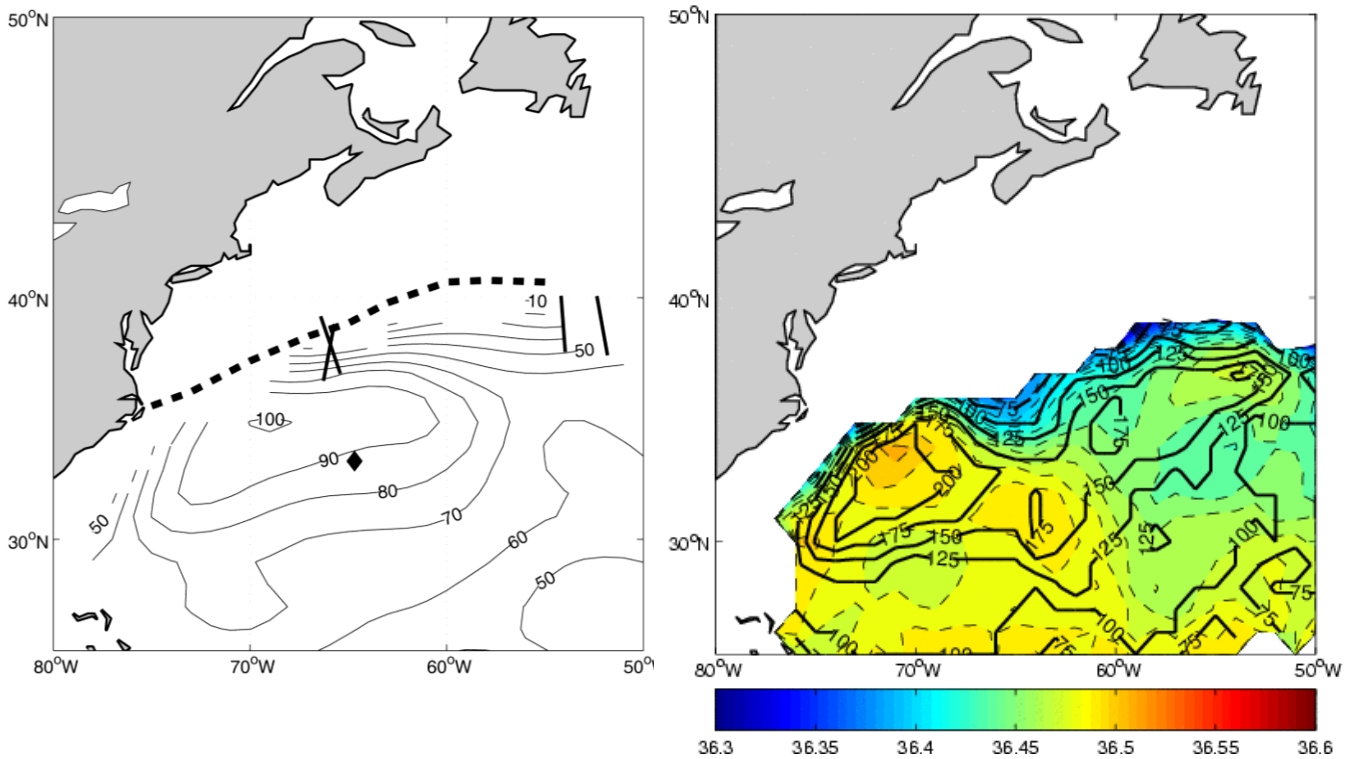
Fig. 2. Left panel: from Kwon and Riser (2004), the geostrophic pressure on the \sigma_{\theta}=26.5 \text{ kg m}^{-3} potential density surface (in cm) based on mean float velocities is plotted with hydrographic lines from the CLIMODE winter cruise of the Knorr in 2007 (thick black lines), the north wall of the Gulf Stream defined by the 200m temperature = 15°C from 1955:2008 (heavy dashed line), and the location of Bermuda (black diamond). Right panel: from the WOCE mean climatology, the thickness of the 17.5:18.5 °C temperature surface (solid black contours) has been plotted for all values exceeding 50m. The color represents the average salinity (psu) in this layer and the contour interval (dashed lines) is 0.01. The thickness and salinity reveal a climatological pattern of EDW variation in the Sargasso Sea.
