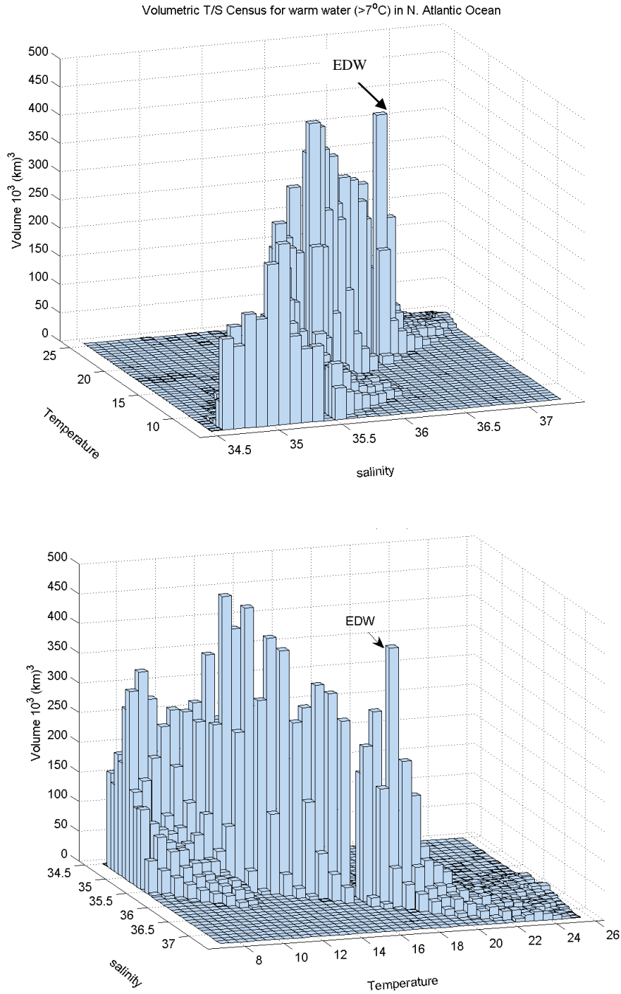
Figure 1. Two different views of a 2D histogram showing the volume (in 10^3 \text{ km}^3 ) of N. Atlantic waters having temperatures > 7^\circ\text{C} , based on the WOCE Global Hydrographic Climatology (Gouretski and Koltermann, 2004). The total volume of EDW bounded by (36.4 – 36.6 psu, 17.5 -18.5 ^\circ\text{C} ) is estimated to be 912 \times 10^3 \text{ km}^3 .
