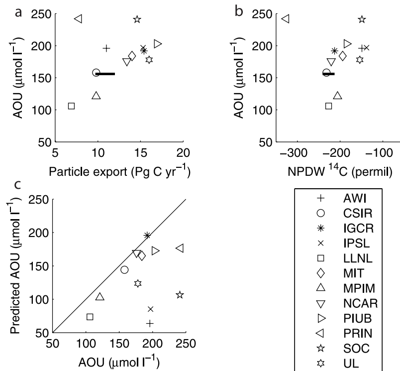
Figure 11. Mean AOU below 2 km as a function of (a) global particle export, (b) North Pacific Deep Water (NPDW) radiocarbon and (c) a box model prediction of AOU based on 2-km particle flux and deep water residence time. Symbols are models. Bars are observations (for AOU and ^{14}\text{C} ) and data-based estimates (for particle export); see text for details.
