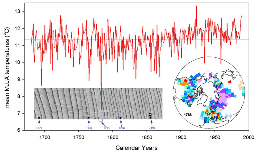
Figure 2. MXD-based Alaskan May–August temperature reconstruction, showing pronounced cold anomaly following the eruption of Laki, Iceland in 1783. Inset at lower left shows annual ring width increments in white spruce from Alaska. MXD measures the peak density value in the latewood of each year. Note very low density in 1783 in this wood section following the eruption of the Laki volcano in Iceland, corresponding to the reconstructed time series. Lower right, spatial anomaly (w.r.t. 1881–1960) plot from BRF98 MXD network [Briffa et al. , 2002]. Figure modified from Jacoby et al. [1999].
