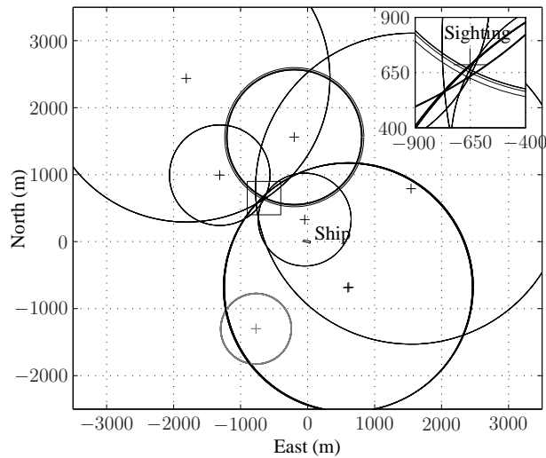
Figure 10: Ship-relative radial constraints on vehicle location during recovery of JAGUAR-02. Ranges at each survey location were acquired from helicopter to an independent relay transponder attached to the vehicle. Both the ship and vehicle were assumed to be lodged in the drifting ice and stationary relative to one another. The one set of inconsistent ranges shown in gray resulted from an erroneous ship's position and required more rangings to discover it than would have otherwise been required to localize the vehicle. The figure indicates a vehicle position of approximately 940 m from the ship's GPS antenna at a heading of 316^\circ true. The vehicle was visually sighted from the helicopter approximately 1 m below the surface in an open lead at the location indicated in the inset on the way to a final ranging location.
