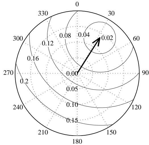
Figure 6: Error surface contours showing the RMS difference between observed and predicted range drift speeds as related to possible ice-drift velocities in compass coordinates for the transponder survey data shown in Fig. 5. The arrow shows the best fit ice drift velocity, 0.14 m/s at a heading of 33° true.
