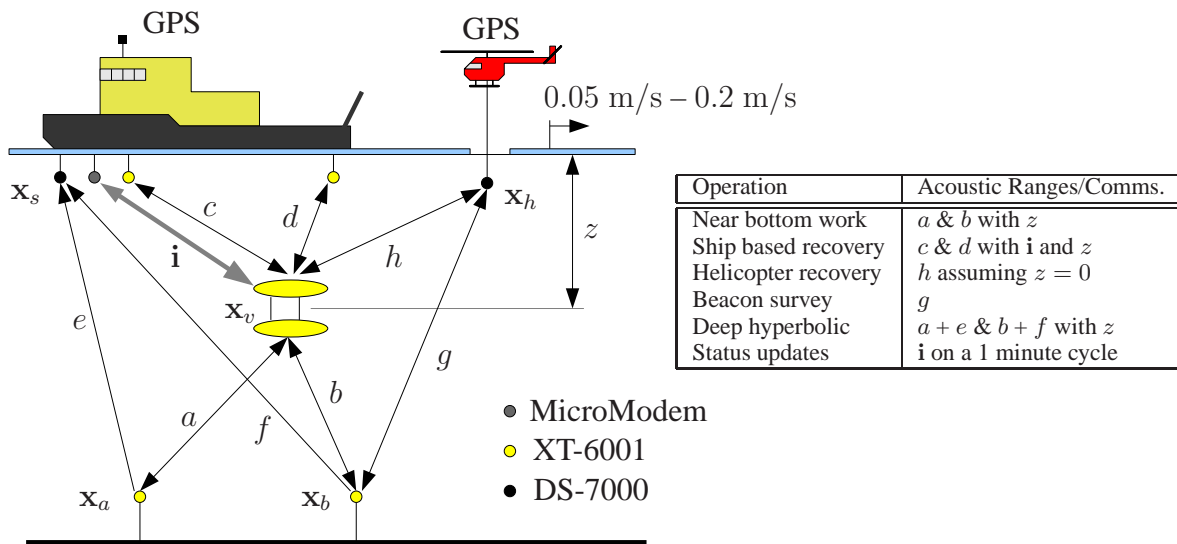
Figure 3: Schematic of the operational setup showing the acoustic ranges employed by the various navigation methodologies reported here (not all concurrently). The vehicle interrogated up to four XT-6001 transponders, two deployed from the ship and two on the bottom. Modem communication (i) was also established between the ship and vehicle. The modem telemetered travel-times and state information recorded on the vehicle to the ship and guidance information from the ship back to the vehicle. The ship's helicopter was used to range to the bottom transponders to survey their initial locations and also on two occasions to localize immobilized vehicles directly beneath the ice. The table summarizes the acoustic paths used during the different positioning operations. The speed range indicates the over-bottom ice drift speeds observed during AGAVE.
