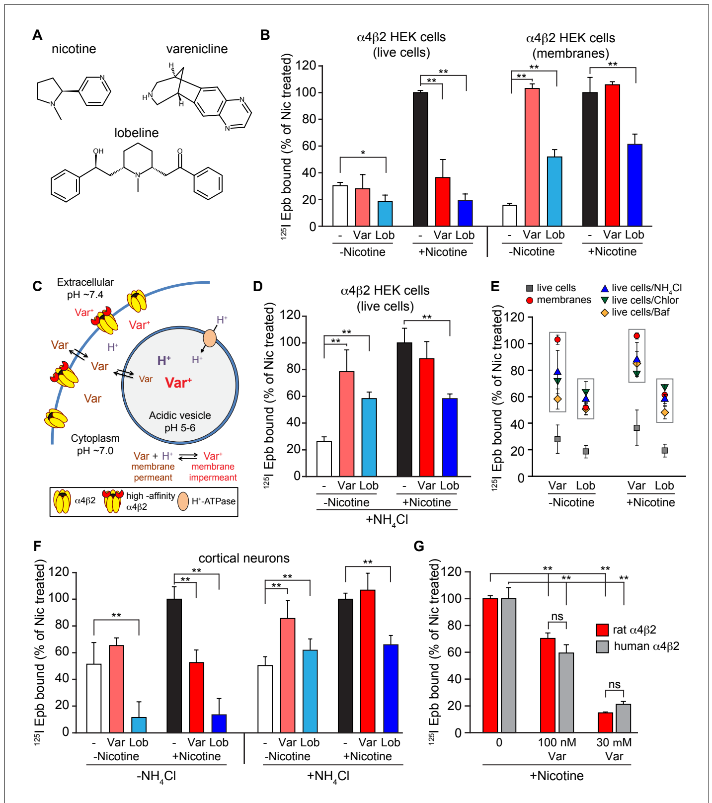
Figure 1. Effect of smoking cessation reagents on \alpha 4\beta 2\text{R} upregulation. (A) Nicotine, varenicline and lobeline chemical structures. (B) Varenicline and lobeline reduced nicotine upregulation of \alpha 4\beta 2\text{Rs} for live cells, but not membranes. ^{125}\text{I} -epibatidine binding performed on live \alpha 4\beta 2\text{R} -expressing HEK cells (left) ( n = 3 ) or membranes (right) ( n = 3 ). Cells were treated for 17 hr with 30 \mu\text{M} varenicline or 30 \mu\text{M} lobeline with or without 10 \mu\text{M} nicotine. Specific epibatidine binding was represented as % of binding relative to nicotine upregulated cells (C) Model of varenicline (Var) trapping in acidic vesicle. Figure 1 continued on next page
