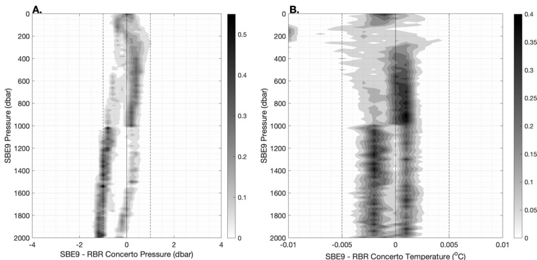
FIG. 3. (a) Pressure differences between SBE9 and the RBR argo^3 's analogous RBR concerto^3 , across all voyages and sensor pairs, after synchronization (see section 3a). Plotted is the frequency distribution in each 20 dbar SBE9 pressure bin, expressed as a fraction of the total pairs in 0.2 dbar increments of the difference. (b) As in (a), but for temperature. Plotted is the frequency distribution in each 20 dbar SBE9 pressure bin, expressed as a fraction of the total pairs in 0.001°C increments of the difference.
