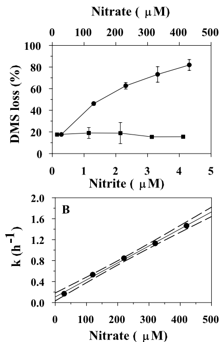
Figure 2. A) Percent DMS photolyzed ( \pm sd) as a function of [nitrate] ( \bullet ) and [nitrite] ( \blacksquare ). 0.2 \mu m-filtered samples were collected Nov. 10, 2003 (65.3 S, 176.8 E) from 10 m and incubated from 1328 to 1438 local time with a 330–380 nm photon exposure of 17.4 \mu Ein \text{cm}^{-2} . Concentrations were monitored by the ^{35}\text{S} -DMS technique with an initial DMS concentration of 1.14 nM. The lowest concentrations in each series represent ambient nitrate (28.6 \mu\text{M} ) and nitrite (0.15 \mu\text{M} ). B) Pseudo first order rate constant for photolysis. The solid line denotes the best-fit employing linear regression analysis ( r^2 = 0.997 , slope = 0.0032 \text{h}^{-1} \mu\text{M}^{-1} , y-intercept = 0.107 \text{h}^{-1} ). Dashed lines denote the 95% CI.
