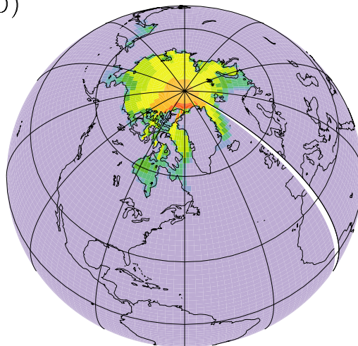
Ice Fraction (2040–2049)
