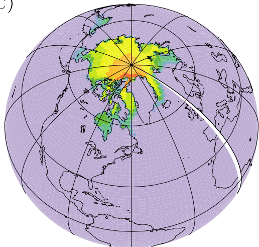
Ice Fraction (2030–2039)
