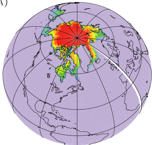
Ice Fraction (1990–2005)
