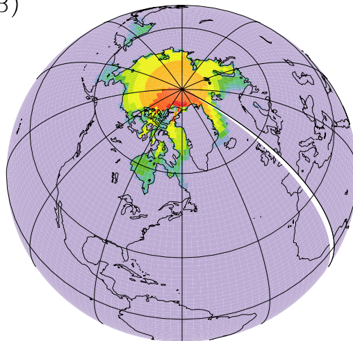
Ice Fraction (2020–2029)
