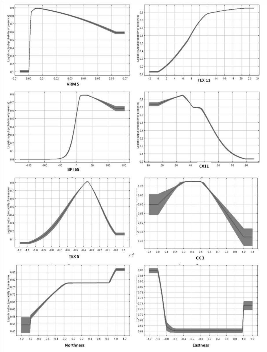
Fig. B 1: Response curves obtained for the Maxent model applied to the SML Province using only the single specified variable to run the model.
