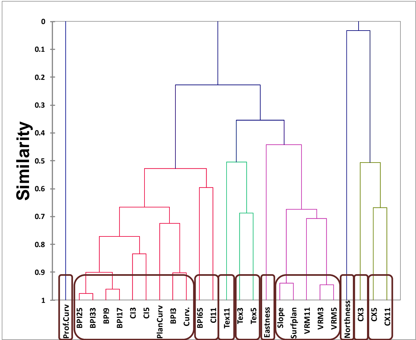
Figure A1 Dendrogram showing groups of correlated terrain variables. Correlated indices have been surrounded. However, the Profile Curvature (Prof.Curv.) was not retained for further analysis, as it is inversely correlated to the BPI3 with a Spearman R coefficient of -0.74.
