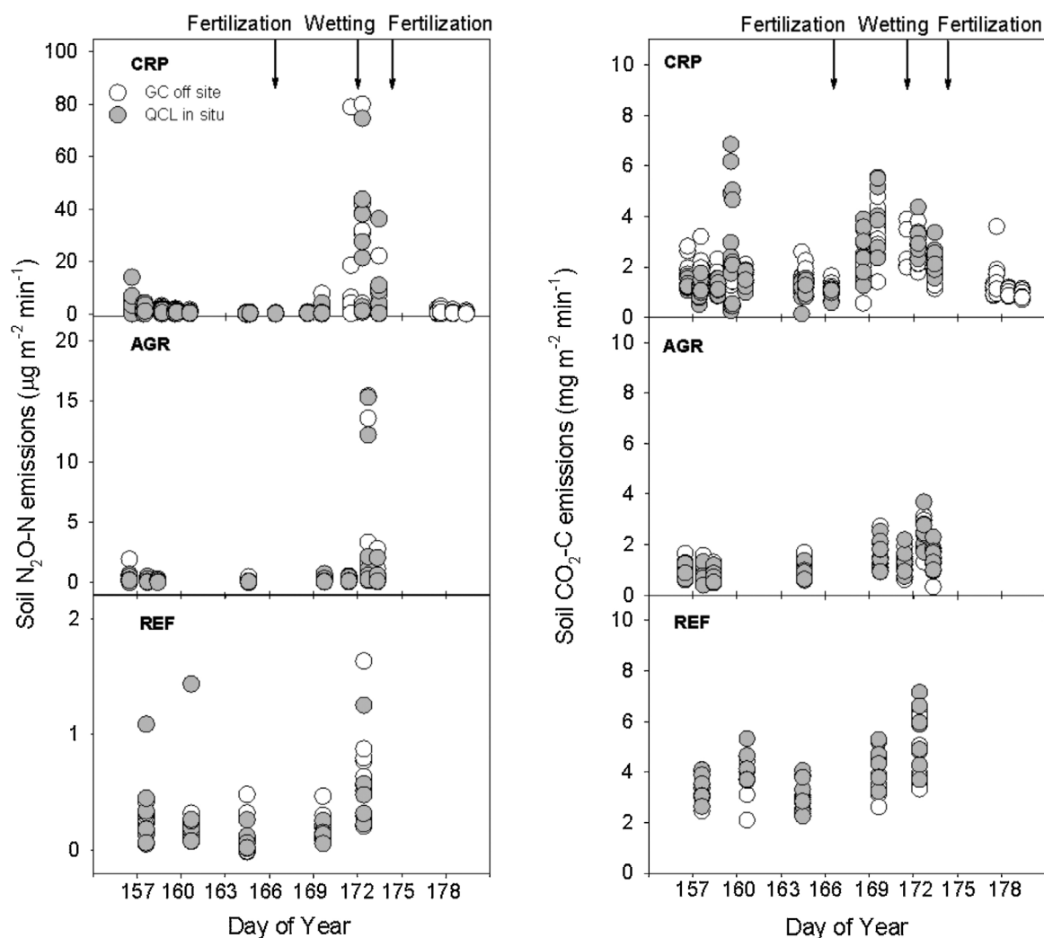
Fig. 3. Soil N 2 O-N ( \mu\text{g m}^{-2} \text{min}^{-1} ; left panel) and CO 2 -C ( \text{mg m}^{-2} \text{min}^{-1} ; right panel) fluxes from individual chambers measured over the study period. Note that the y-axis scale changes between different panels. Arrows indicate the timing of management and the artificial rainfall event.
