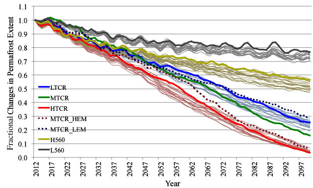
Figure 1. Fractional change in near-surface permafrost extent (poleward of 45°N and in a nonglacier area) with respect to 2012 (around 1.02 \times 10^{13} \text{ m}^2 ) under various climate projections. Thick lines represent the use of climatological geographic patterns in near-surface meteorology throughout the 21st century. Light thin lines represent the inclusion of additional geographic pattern shifts from the IPCC AR4 climate-model projections. The figure legend is detailed in table 1.
