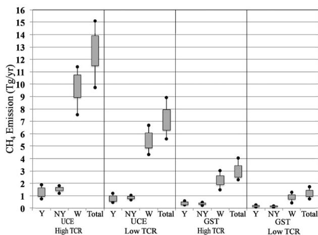
Figure 3. Increases in decadal averaged (2091–2100) annual CH 4 emission (Tg yr -1 , poleward of 45°N) with respect to 2011–20 as a result of the warming and expansion of yedoma lakes (Y), non-yedoma (NY) lakes, wetlands (W), and total inundated areas for the low and high TCR under the UCE and GST scenarios, respectively. Each scenario contains 18 ensemble members (17 members of model-based pattern shifts and one member of climatological pattern). Whisker plots show the minimum, maximum, and plus/minus one standard deviation about the ensemble mean.
