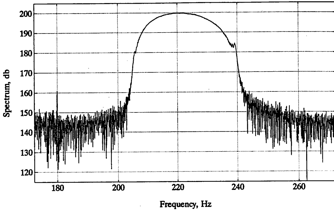
Figure 29: Spectrum of the linear frequency modulated signal with amplitude modulation.
