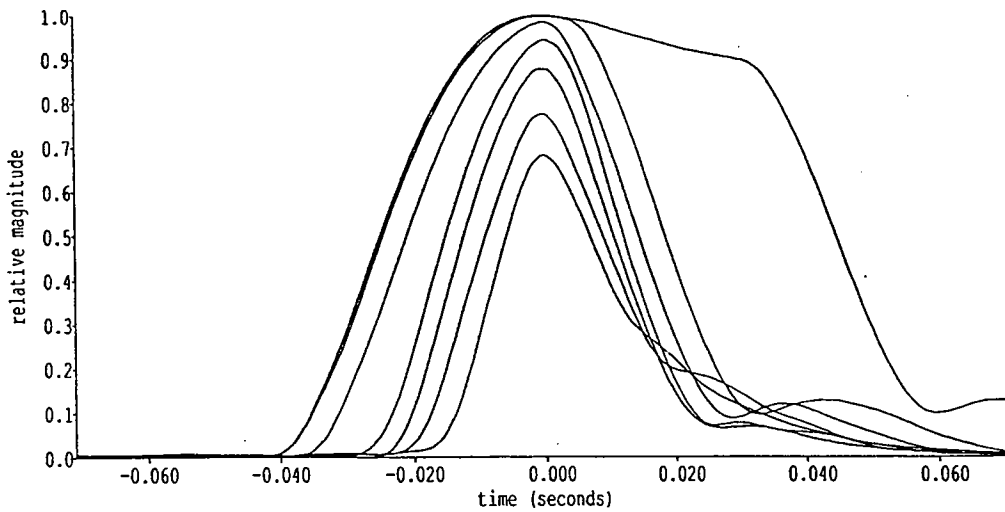
Figure 21: Family of M-sequence convolutions with Q ranging from 3 to 16
