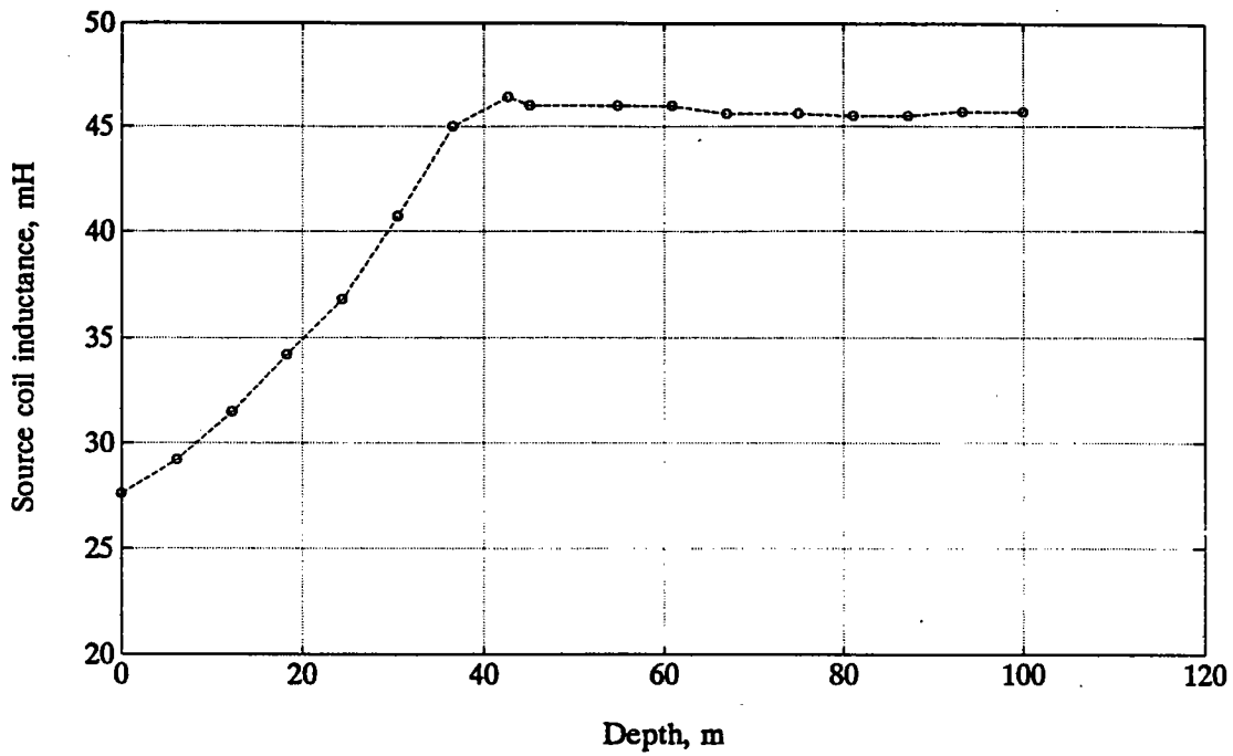
Figure 30: Source coil inductance as a function of depth. Source with pressure compensation system. P_0 = 4 atm, initial pressure inside the compensation system.
