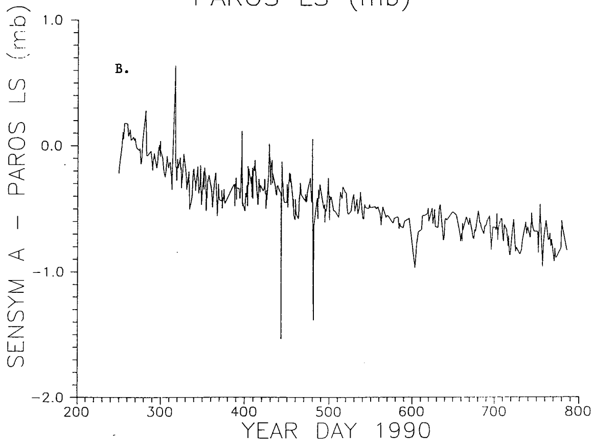
Figures 4A & 4B. A. Sample A of SenSym Model SCX15AN vs PLS. B. Sample A of SenSym Model SCX15AN - difference with PLS us year day.
