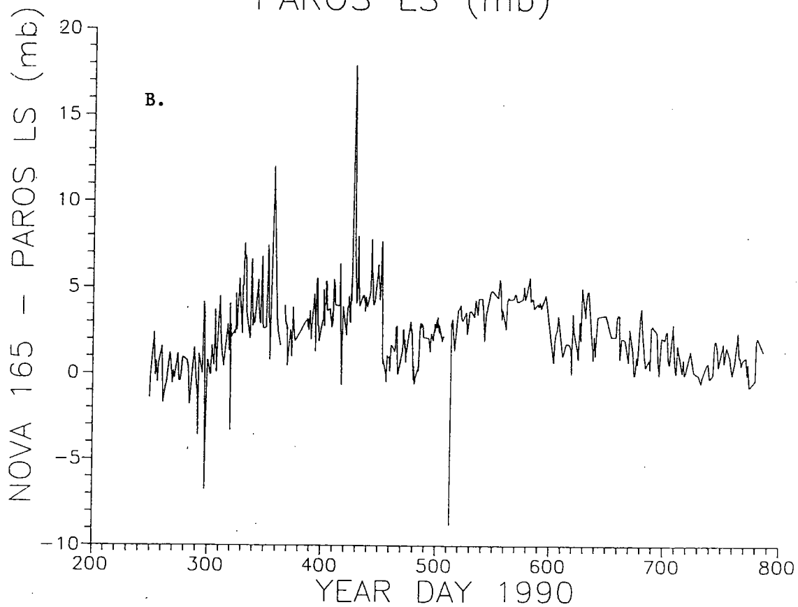
Figure 6A & 6B. A. Sample A of Nova Model PI vs PLS. B. Sample A of Nova Model PI - difference with PLS vs year day.
