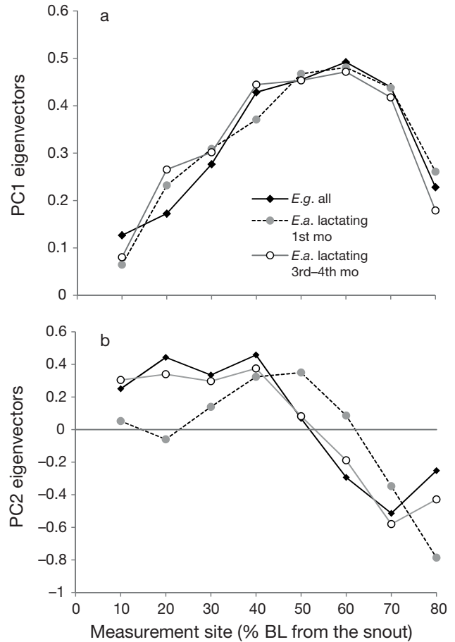
Fig. 2. Eubalaena glacialis and E. australis . Eigenvectors of principal components (a) PC1 and (b) PC2 resulting from the PCA conducted on body width measured using aerial photogrammetry at 10% intervals of the body length (BL) from the snout of 22 E. glacialis ( E.g. ) adult females, and 6 E. australis ( E.a. ) mothers from the initial (July) and later sampling (September, October). E. glacialis was photographed in the Bay of Fundy, Canada, during August 2000, 2001 and 2002; E. australis was photographed in the De Hoop Nature Reserve, South Africa, 1989
