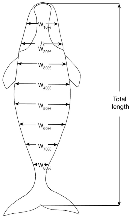
Fig. 1. Eubalaena spp. Diagram of an adult right whale from an overhead perspective showing the features measured using photogrammetry. Body width, W_{x\%} (distance between the lateral edges of the whale's body), was measured at sites located every 10% of the whale's length from snout to fluke notch. Diagram represents stylistic right whale that accurately shows locations of measurement sites but is drawn without regard to nutritional status at any particular life history stage
