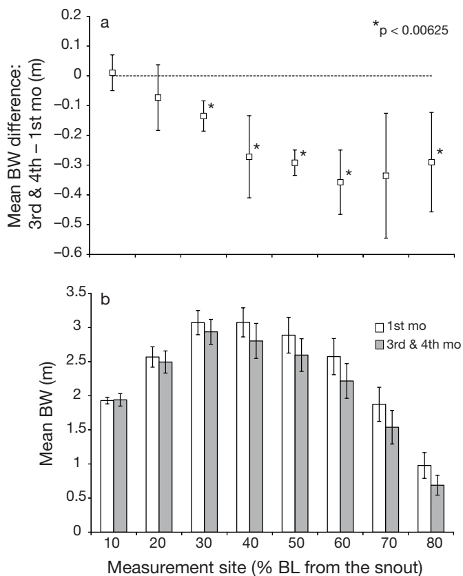
Fig. 4. Eubalaena australis . Comparison of body width (BW) measured every 10% of the body length (BL) from the snout using aerial photogrammetry on 6 E. australis mothers between the first (July) and third or fourth (September, October) month of lactation, De Hoop Nature Reserve, South Africa, 1989. (a) Mean \pm SD difference in BW (m). Asterisks (*) indicate that the mean difference is significantly different from zero ( p < 0.00625 ). (b) Mean \pm SD BW (m)
