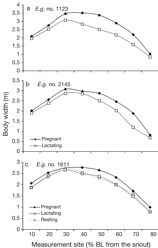
Fig. 6. Eubalaena glacialis . Body width measured every 10% of the body length (BL) from the snout using aerial photogrammetry on 3 females sampled in multiple years at different stages of the reproductive cycle, Bay of Fundy, Canada, August 2000, 2001 and 2002. E. glacialis (E.g.) numbers refer to individual whale identification numbers in the North Atlantic Right Whale Identification Catalog (Hamilton et al. 2007)
