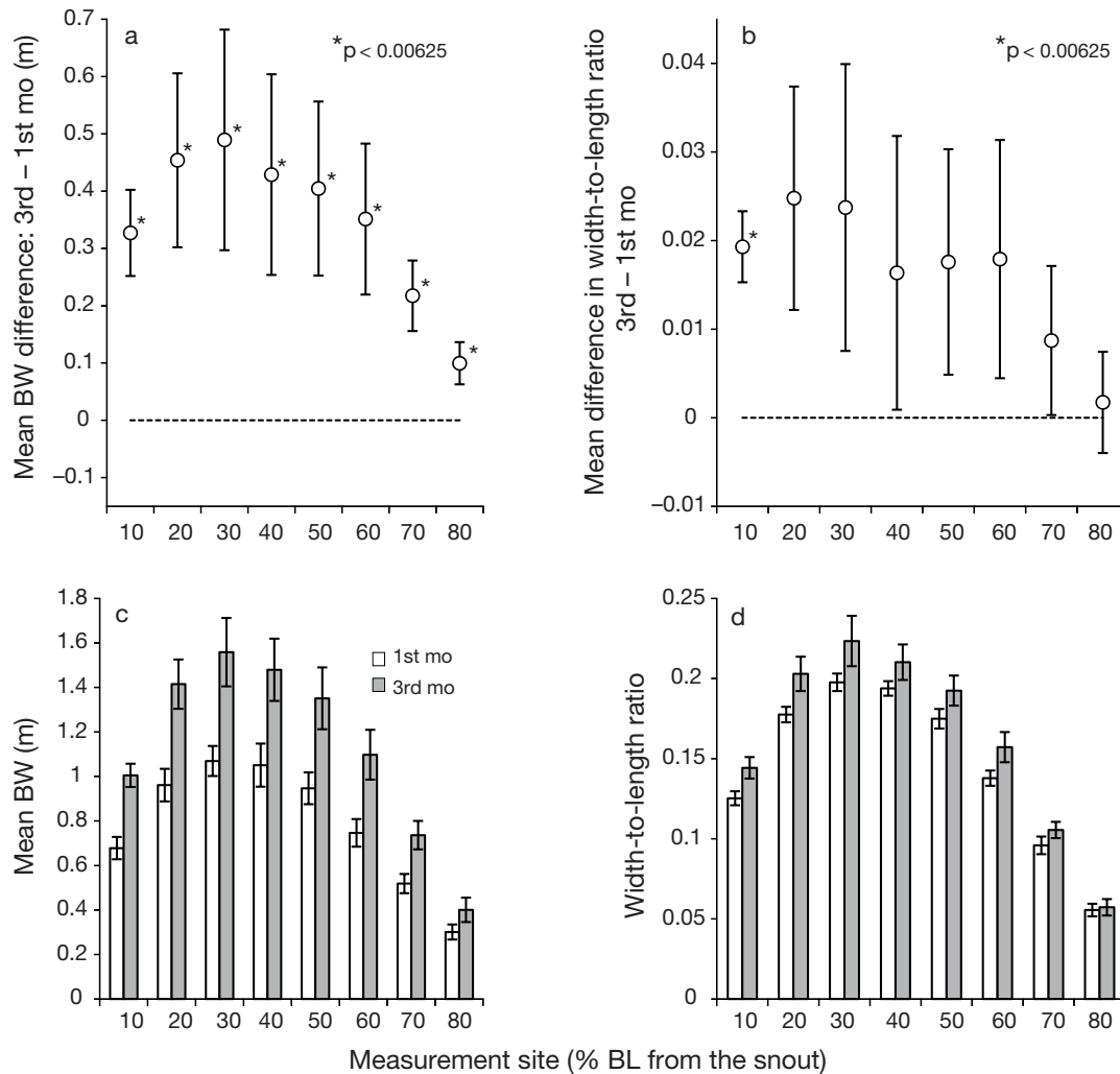
Fig. 5. Eubalaena australis . Comparison of body width (BW) measured every 10 % of the body length (BL) from the snout using aerial photogrammetry on 5 calves between the first (July) and third (September) month of suckling, De Hoop Nature Reserve, South Africa, 1989. Mean \pm SD in (a) difference in BW (m), (b) difference in body width-to-length ratios, (c) BW (m) and (d) body width-to-length ratios. Asterisks (*) indicate that the mean difference is significantly different from zero ( p < 0.00625 )
