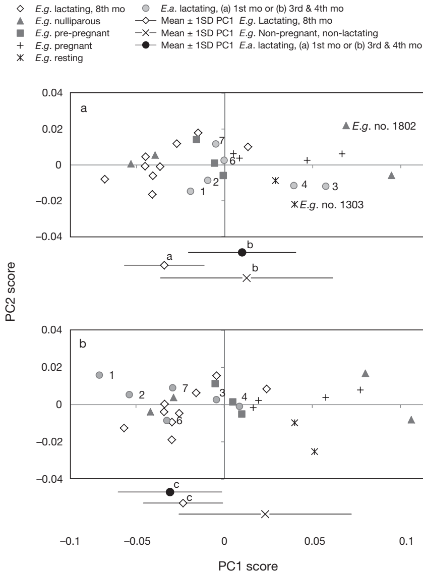
Fig. 3. Eubalaena glacialis and E. australis . Principal components (PC) scores for PC1 and PC2 generated from PCAs conducted on aerial photogrammetric measurements of right whale body width-to-length ratios collected at 10% intervals of the body length from the snout. E. glacialis ( E.g. ) was photographed in the Bay of Fundy, Canada, during August 2000, 2001 and 2002; E. australis ( E.a. ) was photographed in the De Hoop Nature Reserve, South Africa, 1989. (a) PC1 and PC2 scores for adult female E. glacialis of differing reproductive status and for E. australis mothers measured in July (the first month of lactation). Each E. australis mother is labeled with a number (1–4, 6, 7); 2 E. glacialis females are labeled with their individual whale identification numbers from the North Atlantic Right Whale Identification Catalog (Hamilton et al. 2007). (b) PC1 and PC2 scores from the same series of body width-to-length ratios from the adult female E. glacialis combined with the series from the later sampling (September–October, third to fourth month of lactation) of the same E. australis mothers. The E. australis mothers are labeled with the same numbers assigned to them in (a). Mean \pm SD of PC1 scores for lactating and non-pregnant, non-lactating E. glacialis and for the E. australis mothers are shown below the panel in both (a) and (b); means with the same letter are not significantly different at (a) \alpha = 0.025 or (b) \alpha = 0.05
