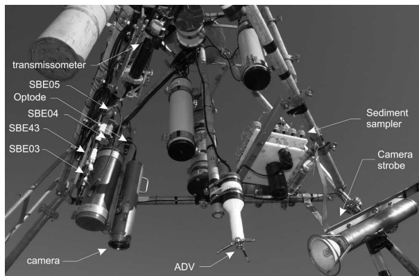
FIG. 1. View of tripod 717 from below the frame showing the locations of the Aanderaa optode and the Sea-Bird sensors. Also deployed on this tripod are an SBE04 conductivity cell, SBE43 oxygen sensor, SBE05T pump, and SBE03F temperature cell, a Sontek acoustic Doppler velocimeter, a Benthos still camera, Sea Tech transmissometer, a sediment sampler, and an RDI ADCP (not visible).
