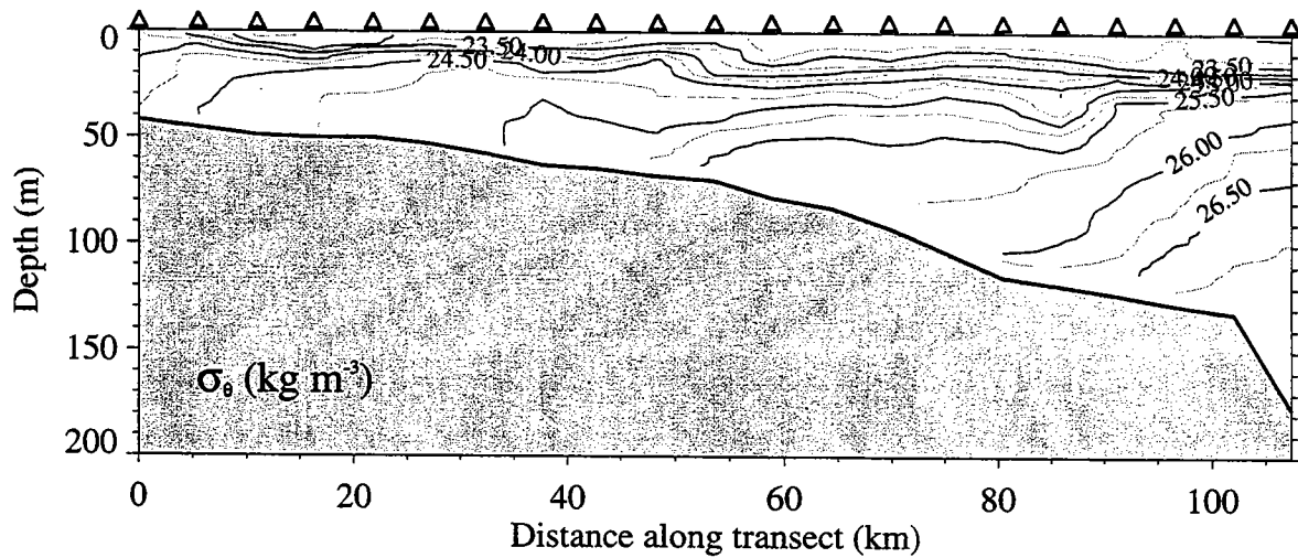
Figure IV.3. Across Shelf CTD Section on 8/04/96.
