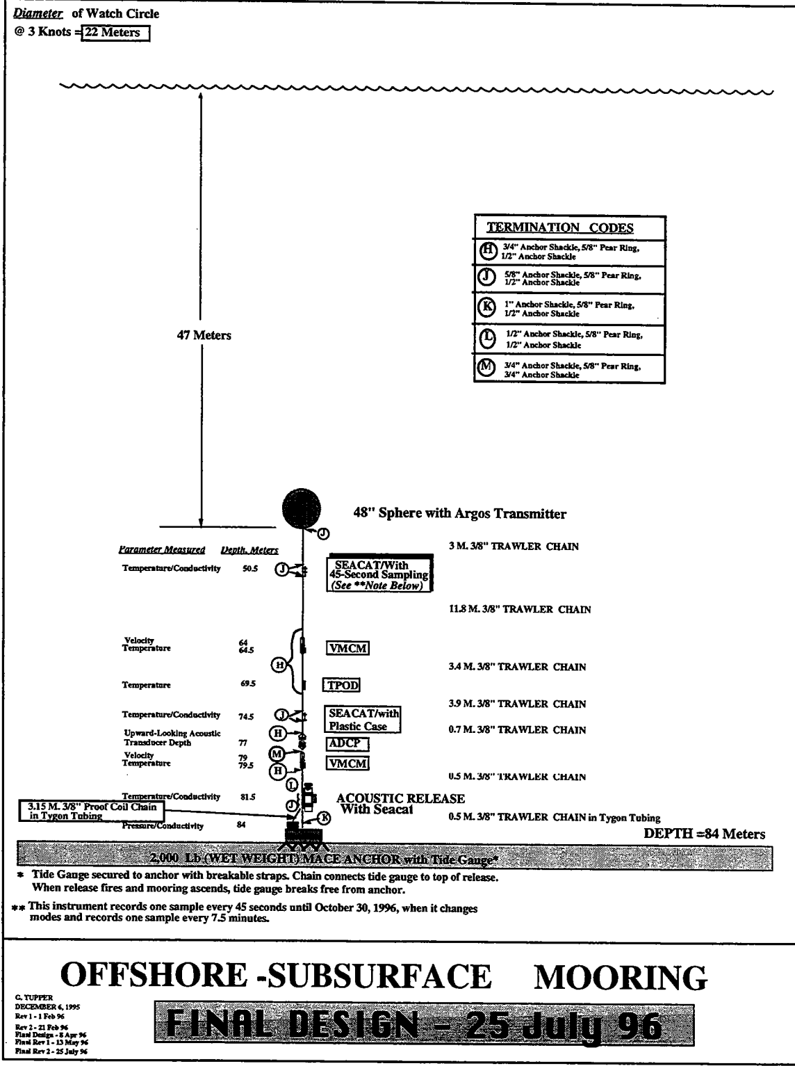
Figure III.B.10: Offshore Subsurface Mooring Diagram.
