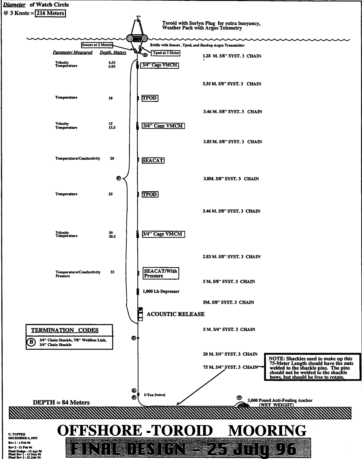
Figure III.B.9: Offshore Toroid Mooring Diagram.
