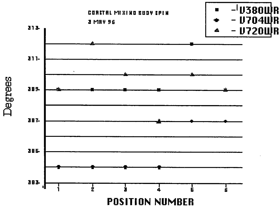
Figure III.C.3. Buoy Spin Results.
