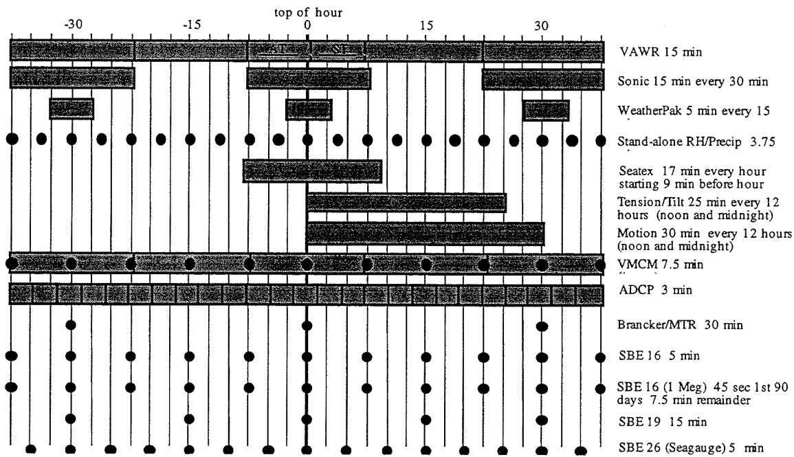
Figure III.C.1. Instrument Timing Schematic.
