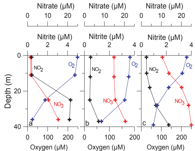
Fig. 7. Vertical profiles of \text{O}_2 , nitrate (including nitrite) and nitrite at three shallow stations located over the Omani shelf: (a) Sta. SK209/09 ( 21.118^\circ N, 59.149^\circ E), (b) Sta. SK209/13 ( 19.838^\circ N, 58.343^\circ E), and (c) Sta. SK208/15 ( 18.661^\circ N, 57.192^\circ E).
