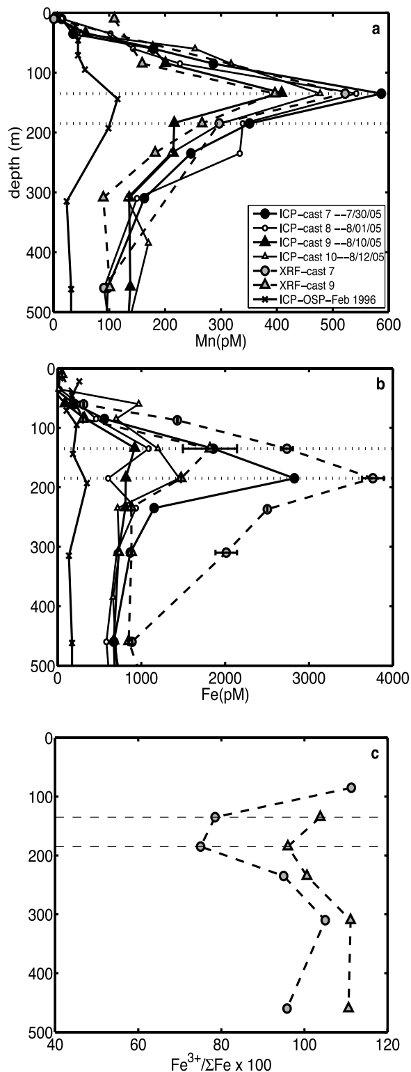
Figure 1. Concentration profiles of particulate (a) Mn and (b) Fe as determined by ICP-MS on the acid leachable (labile) fraction (solid line), and by synchrotron XRF (total) (dashed lines, grey symbols) in the 1–51 \mu\text{m} particle size fraction. Acid-leachable concentrations from Ocean Station Papa (OSP) in the ESP [Lam et al. , 2006] shown (solid lines, X symbols) for comparison. Error bars on XRF Fe, where present, indicate standard deviations of samples analyzed twice. (c) Profiles of the redox ratio of particulate Fe, expressed as Fe^{3+}/\Sigma Fe \times 100 , showing a minimum in oxidation state at 185 m. See Table S1 for analysis details. The depths of Mn_p and Fe_p maxima are shown as large horizontal dashes in all profiles.
