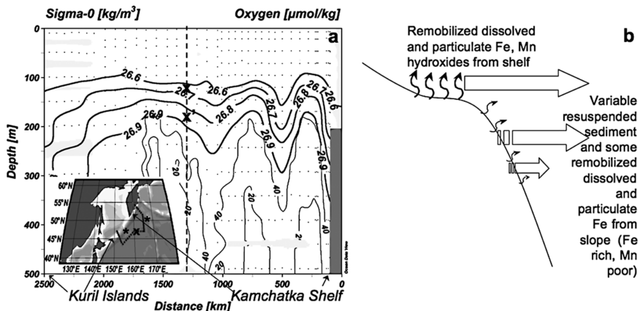
Figure 2. (a) Potential density (thick contours) and dissolved oxygen (thin contours) sections constructed from three WOCE cruises connecting the Kamchatka peninsula (right third: P13-August 1992), station K2 (vertical dashed line; middle third: P1-August 1985), and into the Sea of Okhotsk through the Kuril Straights (left third: P01W-September 1993) [Schlitzer, 1996], showing that the density surfaces on which the Mn_p (x) and Fe_p (x') peaks lie intersect with the continental shelf and upper continental slope of Kamchatka and the Kuril Islands and are shallower than the core of the oxygen minimum zone ( 20 \mu\text{mol/kg} ). This composite section is merely illustrative and is not meant to imply a particular pathway for delivery of Mn and Fe. Locations of closest available dissolved Fe profiles from Nishioka et al. [2003] and Brown et al. [2005] marked with *. (b) Schematic of Mn and Fe delivery from continental shelf and slope to open ocean, showing a constant shelf source of remobilized Mn and Fe from the shelf, and a more variable source of Fe remobilized and resuspended from slope sediments.
