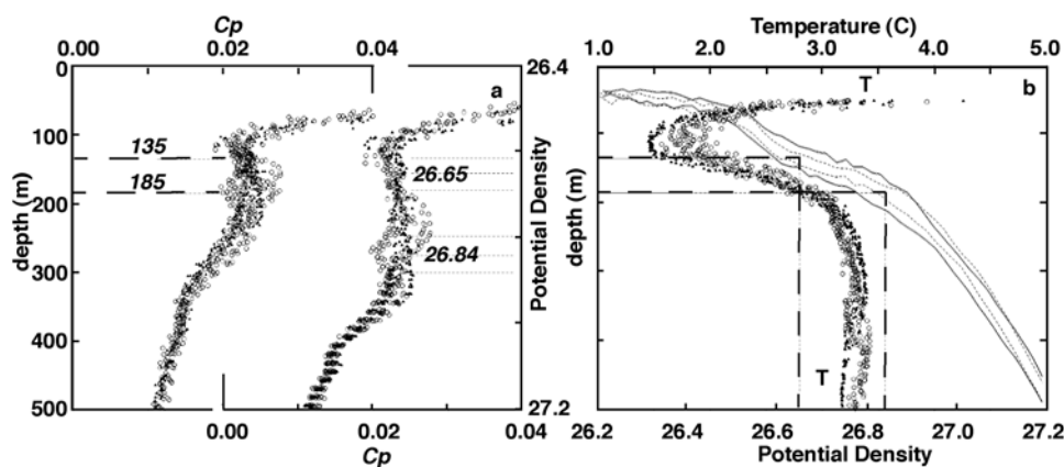
Figure 3. Data from 13 CTD profiles bracketing pairs of MULVFS casts: 1st set (Jul 30–Aug 2) shown as open circles; 2nd set (Aug 10–12 2005) shown as smaller closed triangles. (a) Particle beam attenuation coefficient ( C_p ) plotted against depth (left) and potential density (right) showing more variable particle concentrations above and below 135 m. Mn_p and Fe_p phases are minor contributors to the C_p signal which is dominated by organic matter [Bishop et al. , 2004]. C_p values in waters shallower than 50 m were as high as 0.2 (not shown). (b) Depth profiles of temperature (symbols) and potential density (solid and dotted lines denote depth range of potential density surfaces during the 1st and 2nd sets, respectively). Isopycnal displacements of \sim 40 \text{ m} were evident in the 1st set. The relatively large variability for Fe near 185 m is consistent with C_p data and indicates a more variable upper continental slope source. Dust delivered material would not exhibit such depth dependent variability.
