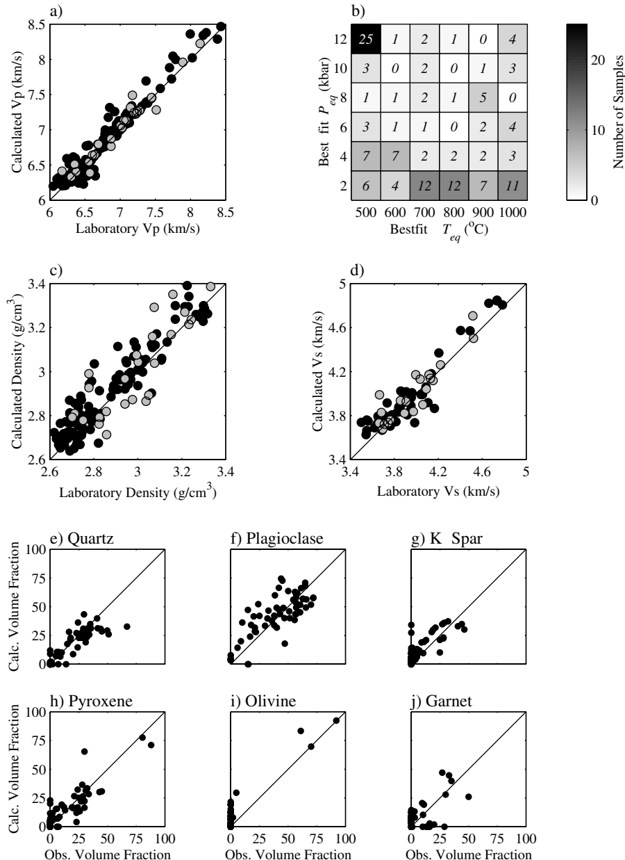
Figure 5. Comparison of calculated and laboratory determined V_p in 139 igneous and meta-igneous rocks at T_{ref} = 25^\circ\text{C} and P_{ref} \geq 6 kbar [Manghnani et al. , 1974; Kern and Richter, 1981; Kern and Schenk, 1985; Christensen and Szymanski, 1988; Kern and Schenk, 1988; Christensen, 1989; Burke and Fountain, 1990; Fountain et al. , 1990; Kern and Tubia, 1993; Miller and Christensen, 1994]. V_p , V_s , and density are calculated for each bulk composition from the equilibrium mode over a range of T_{eq} = 500\text{--}1000^\circ\text{C} and P_{eq} = 2\text{--}12 kbar. The best-fit V_p is then determined for each sample over the range of equilibrium conditions. (a) Best-fit V_p versus experimentally determined V_p . For experimental data in which velocities were measured in multiple directions the average value is used in the comparison. Gray symbols represent samples containing garnet, black symbols represent samples that are garnet-free. The residuals of the best-fit data are calculated relative to a one-to-one correlation (black line), and have a mean = 0.047, median = 0.015, and standard deviation = 0.125 km/s. (b) 2-D histogram of best-fitting T_{eq} and P_{eq} . Italic numbers indicate number of samples in each bin. (c) Calculated versus laboratory measured density using the equilibrium modes fit for V_p (mean = 0.038, median = 0.032, and standard deviation = 0.080 \text{g/cm}^3 ). (d) Calculated versus laboratory V_s using equilibrium modes fit for V_p (mean = 0.037, median = 0.036, and standard deviation = 0.114 km/s, N = 66 ). (e)–(j) Comparison of major minerals in calculated and observed modes for samples on which point-count analyses were performed ( N = 50 ).
