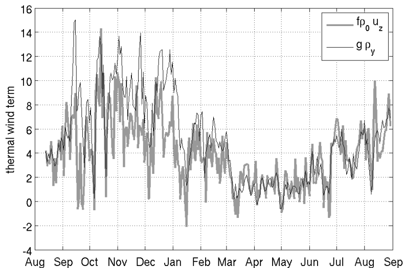
Figure 10 Time evolution of the vertical shear in the along-strait flow direction and of the horizontal density gradient at 60m at mooring B (units are 10^{-4} \text{ kg}/(\text{m}^3 \text{ s}^2) ).
