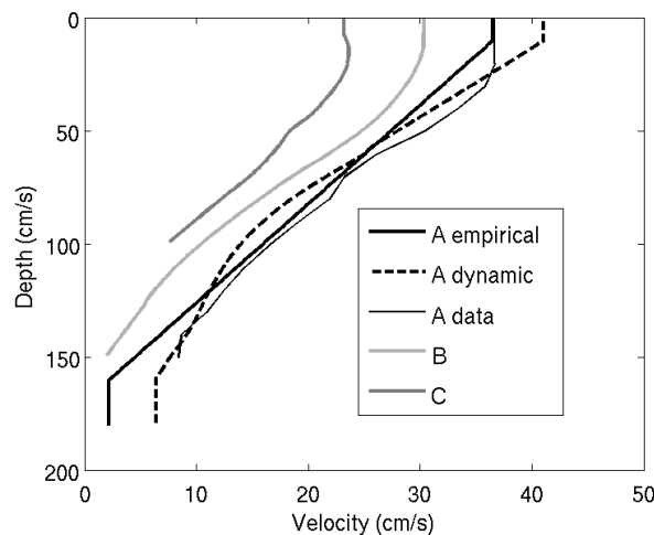
Figure B2 Temporally averaged (over one year) along-strait velocity at A using the empirical and dynamic methods described in the text. Also shown are the yearly average velocities at B and C, and that observed during the 21 days of ADCP operation at A.
