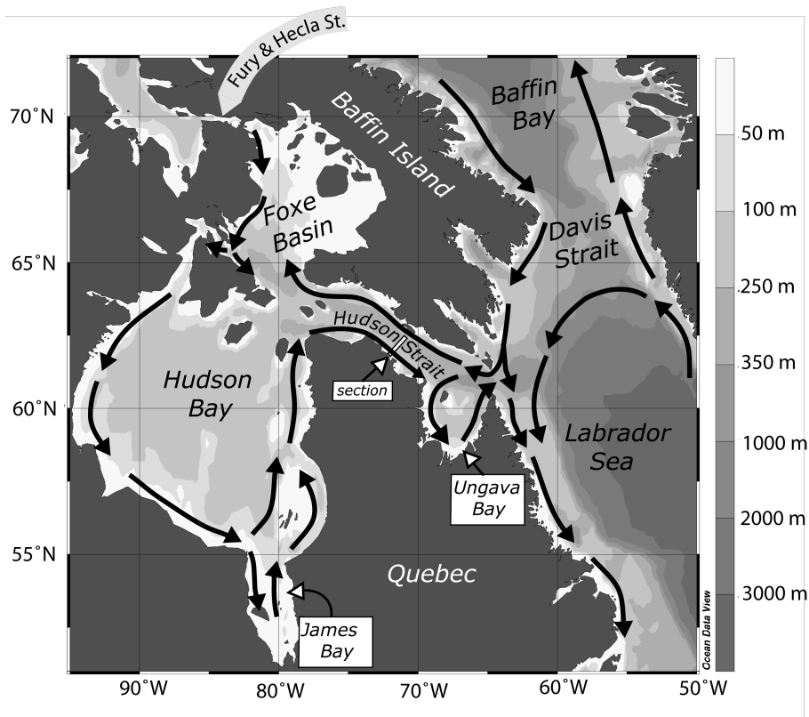
Figure 1. Hudson Bay System: bathymetry and schematic circulation.
