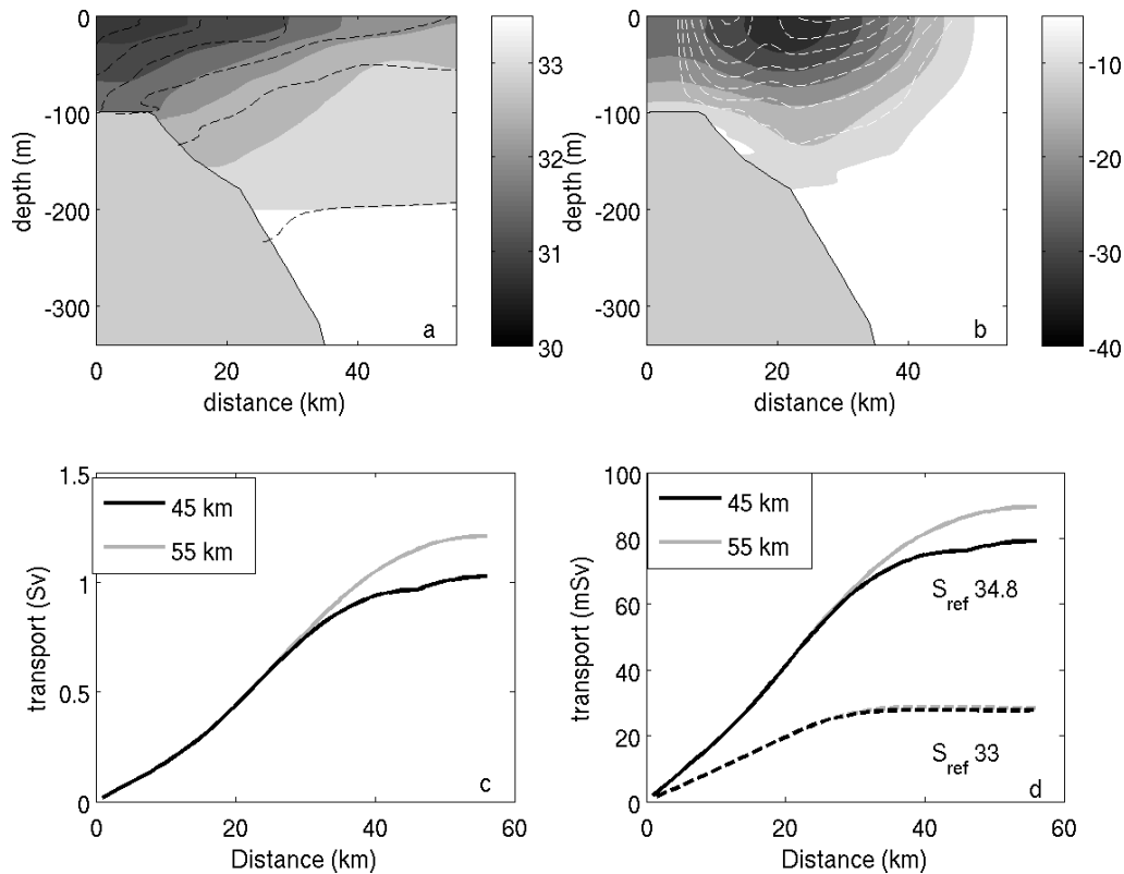
Figure 14: a) Reconstructed mean salinity, overlaid are the same salinity contours (dashed lines) from the hydrographic section of August 2005; b) Reconstructed mean velocity, overlaid are the geostrophic velocity contours (assuming zero velocity at the bottom, dashed white – same contour interval) from the reconstructed mean salinity (see text); c) Cumulative volume transport as a function of distance from coast; d) same as c) but for freshwater transport.
