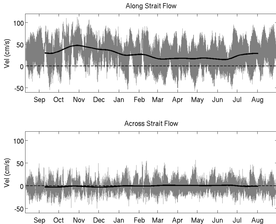
Figure 7. Along and across strait flow at 40m at B. Two month low pass filtered time series is overlaid in bold.
