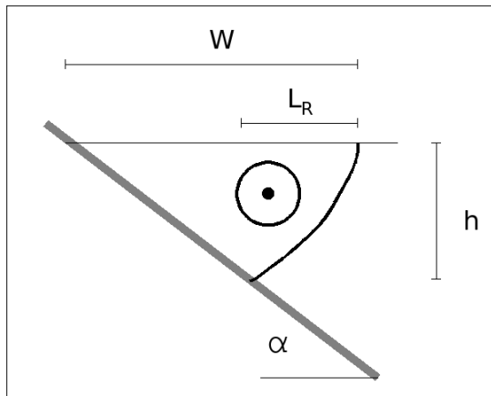
Figure 11 – Schematic of the structure of a buoyant, gravity current over sloping topography (redrawn from Lentz and Helfrich, 2002).
