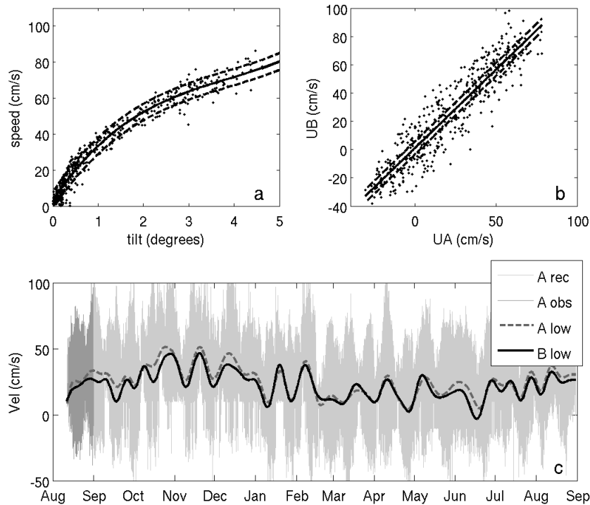
Figure B1 Reconstruction of the along strait flow at 60m at A: a) along strait flow at A at 60m (from the short ADCP record) versus tilt of the mooring. Also shown is the cubic fit with the 95% confidence intervals. b) relation between the along strait velocities at 60m at A and at B, the linear fit is superimposed. c) Reconstructed flow field at 60m at A. Overlaid are: the short observed record from A, and the two week low pass filtered for the observed record from B and the reconstructed field from A.
