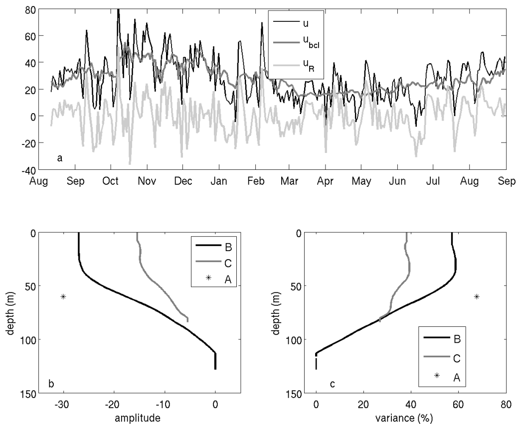
Figure 12 a) Decomposition of the along strait flow at 40m at B (black) into a baroclinic component which covaries with density (dark grey) and a residual (light gray). The baroclinic component is shifted by an amount equal to the average mean flow over the record to differentiate the two, b) Amplitude function \beta(z) (see text) as a function of depth for C, B and at 60m at A, c) Fraction of the variance explained by the baroclinic flow for the same data as in b) as a function of depth.
