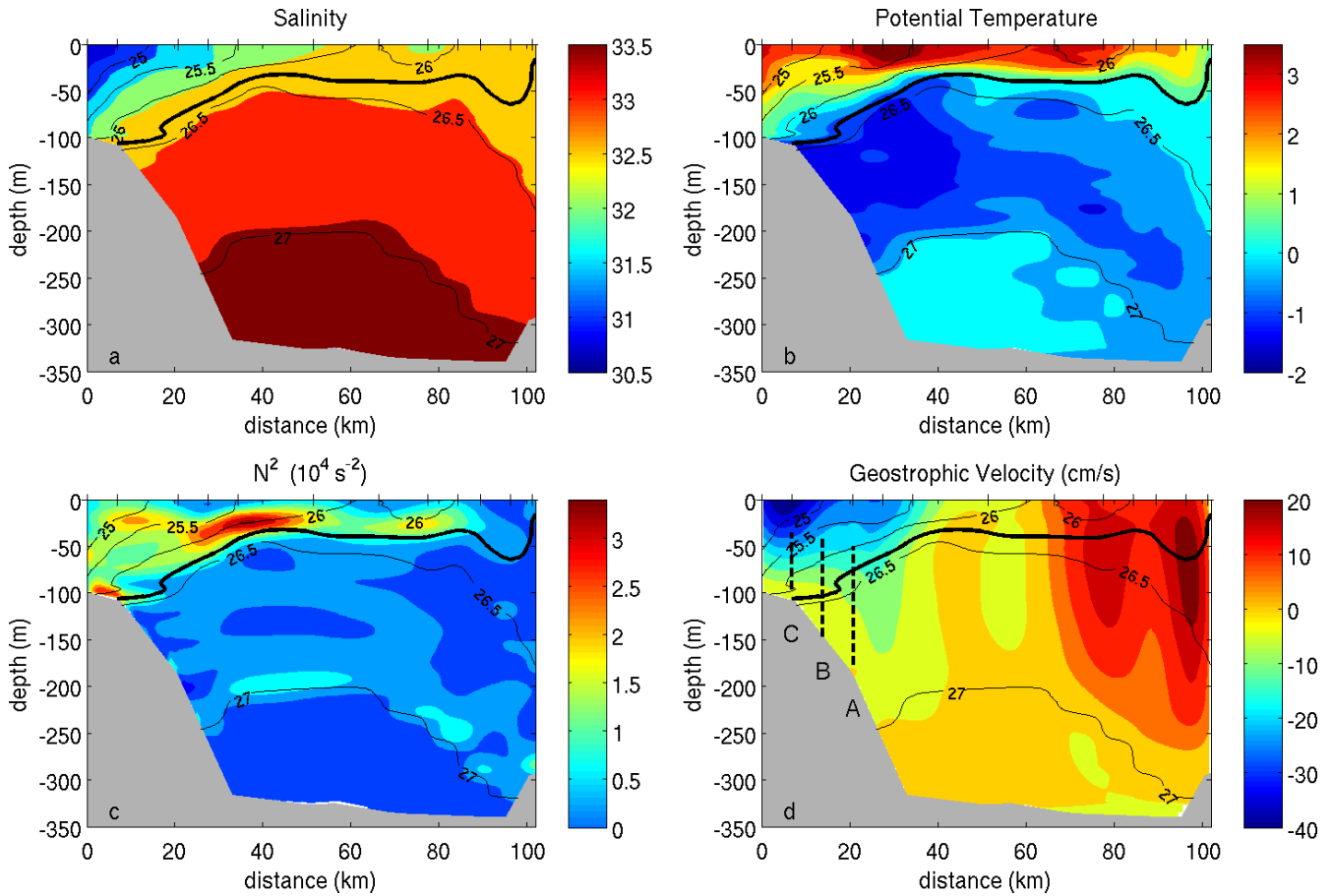
Figure 2. a) Salinity b) potential temperature ( ^\circ\text{C} ) c) Brunt-Vaisala frequency squared and d) geostrophic velocity, from a hydrographic survey across the strait in September 2005, isopycnals are overlaid on all panels, with the \sigma_t = 26.4 in bold. Station location is indicated at the top of each plot. The three mooring locations are shown in d).
