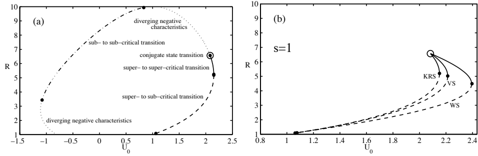
Figure 2: (a) Full solution space for the KRS theory with r = 0.1 and s = 1 . (b) Allowable solution space for KRS, WS and VS theories for r = 0.1 and s = 1 . Line type indicates behavior of characteristics as marked in (a).
