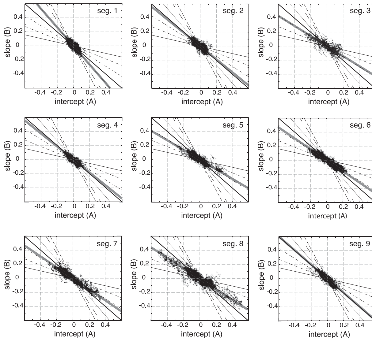
Figure 8. A versus B crossplots obtained for the nine fourth-order AML segments within the analysis windows outlined in Fig. 7(a). Each CRP gather gives rise to several ( A , B ) pairs, of which only one is generated by the negative excursion of the AML waveform at vertical incidence (others are from positive excursions, and noise above and below the AML). The best-fit trend is plotted with a thick solid grey line. Calculated trend lines from the template are shown as in Fig. 4.
