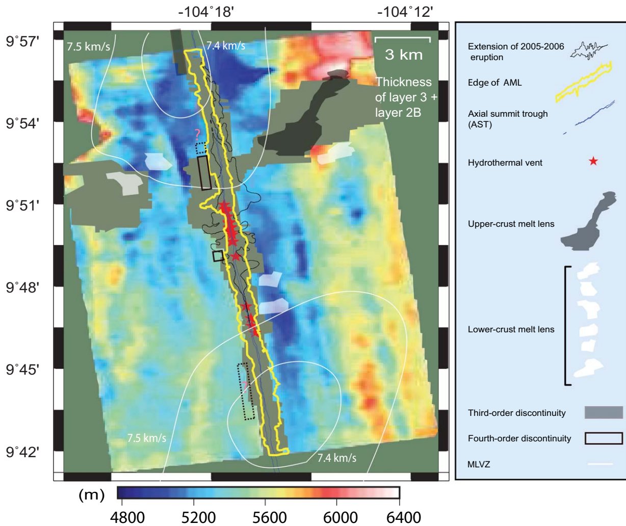
Figure 11. Crustal thickness from Figure 7d after removing layer 2A is shown together with the location of magmatic segmentation, hydrothermal activity, MLVZs, OAMLs, AML, AST, and extent of 2005–2006 volcanic eruption. Black dotted rectangles with red question marks are locations of disputed discontinuities. Source of information is same as in Figures 1 and 9.
