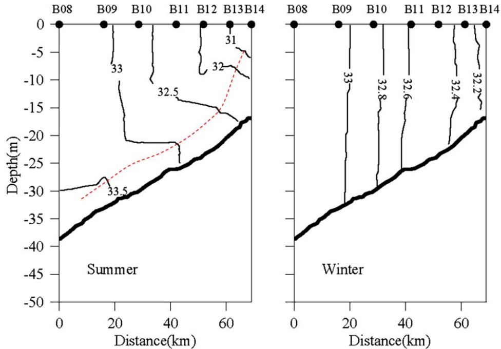
Figure 4. Summertime and wintertime salinity distributions on transect B08-B14 in the northern Gulf of Tonkin measured during hydrographic surveys made in summer and winter, 2006. Red dashed line denotes the height of the bottom boundary layer in the summer season. The salinity data were digitalized from figures listed in Sun et al. [2009].
