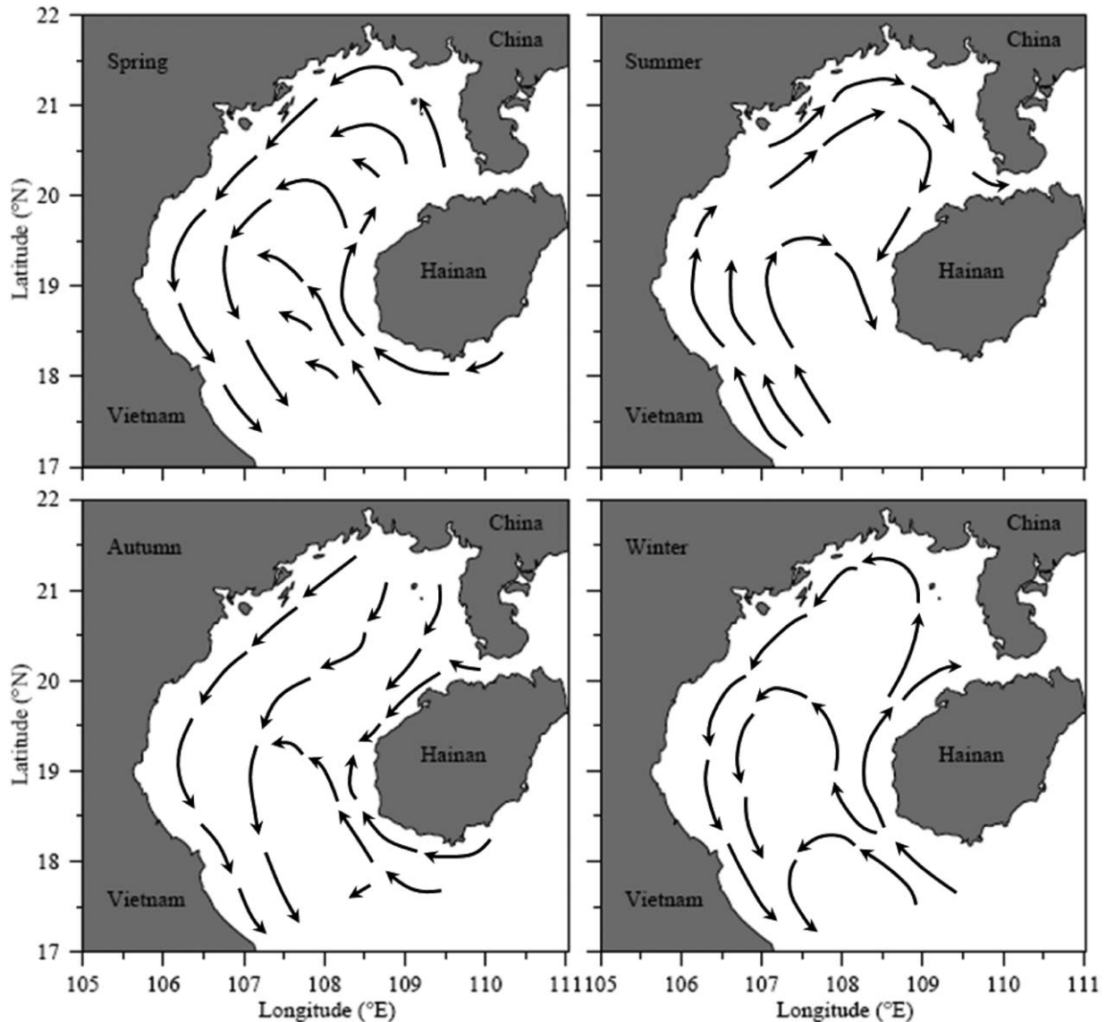
Figure 3. Schematic of the conceptual seasonal circulation patterns in the Gulf of Tonkin based on wind-driven circulation theory with consideration of the 1960s China and Vietnam joint hydrographic survey results.
