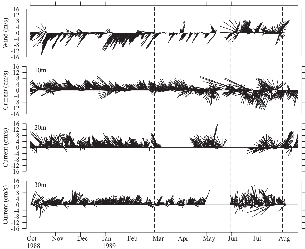
Figure 10. A 33 h low-passed filtered wind vectors at 10 m height and subtidal currents at depths of 10, 20, and 30 m for the period October 1988 to August 1989. Dashed line: the boundary defined for the seasons.
