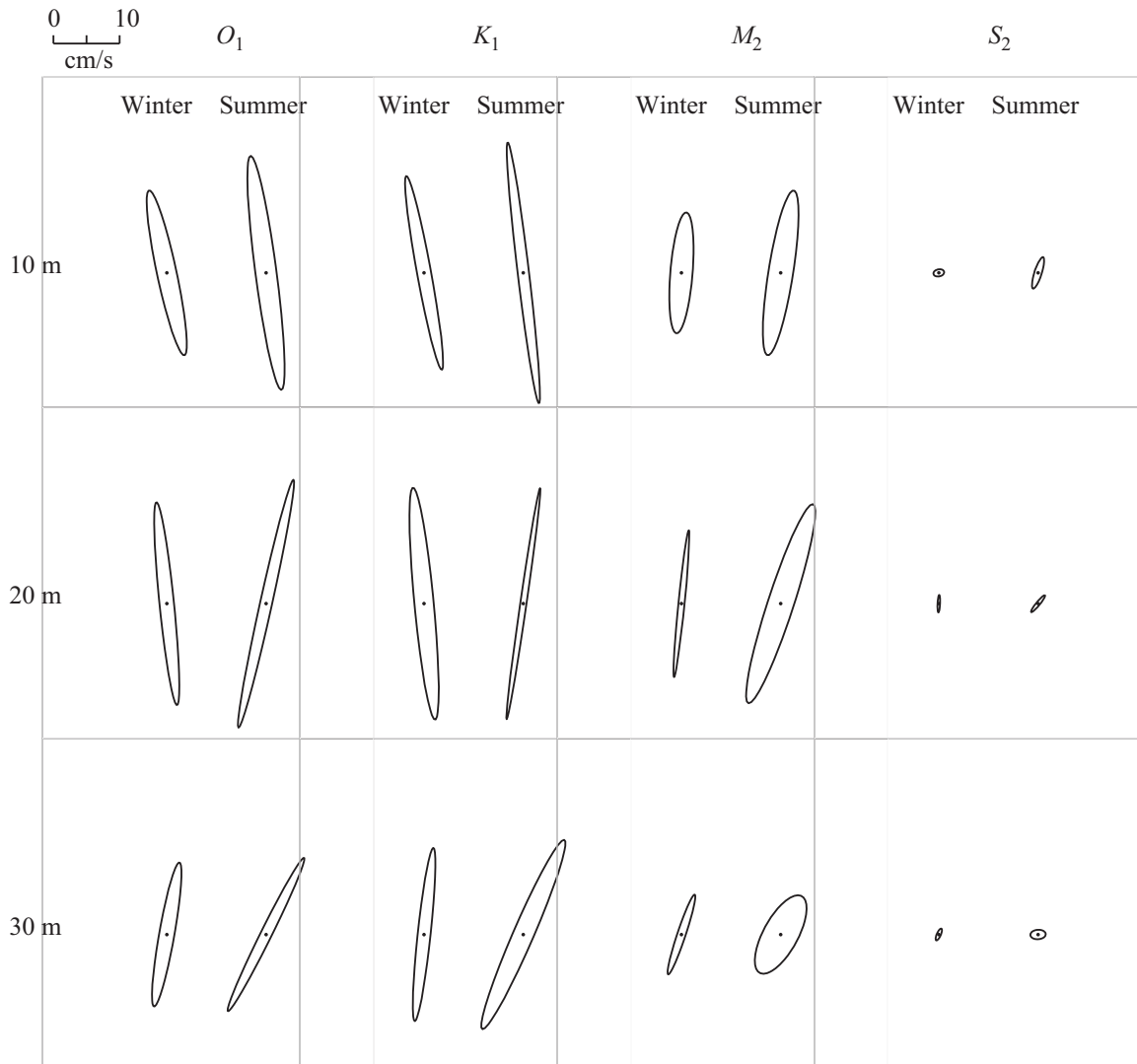
Figure 7. Tidal current ellipses for O_1 , K_1 , M_2 , and S_2 constituents at depths of 10, 20, and 30 m at site A for the winter and summer periods of 1988–1989.
