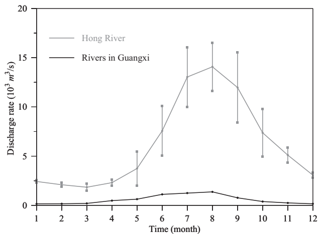
Figure 2. Climatological monthly mean freshwater discharges from the Hong River, Vietnam and rivers along the coast of Guangxi Province, China. Data for the Hong River was from Chen et al. [2012].
