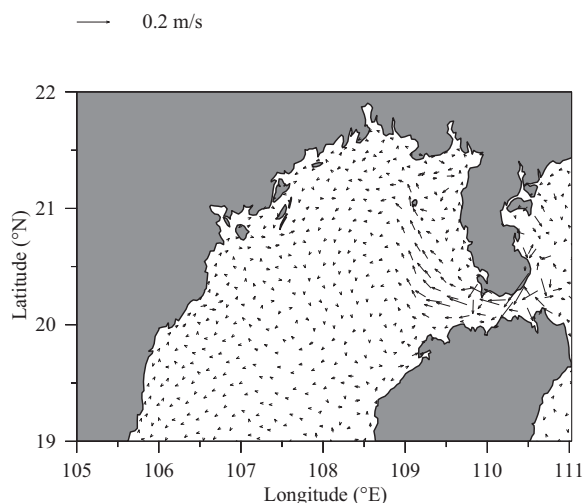
Figure 16. Maps of the monthly averaged current vectors in the northern Gulf of Tonkin for the homogeneous case with only tidal forcing (Ex 2).
