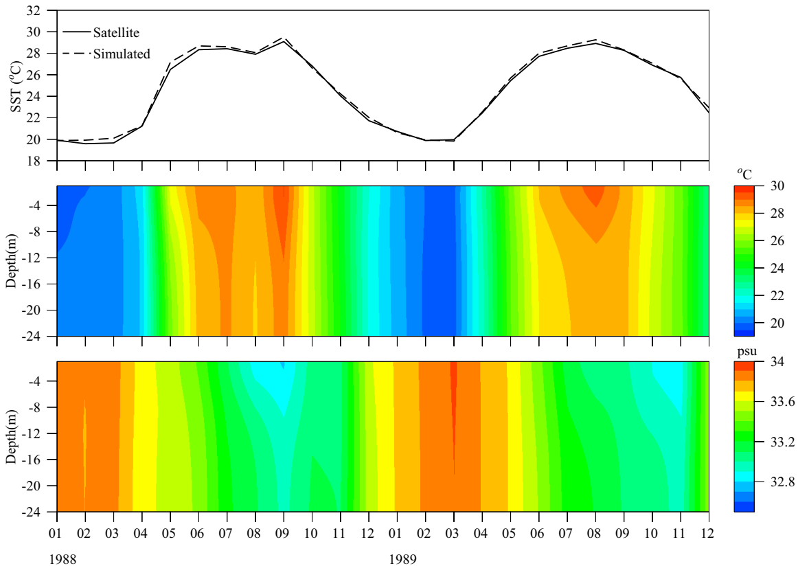
Figure 9. Time series of (top) the satellite-derived sea surface temperature (SST) and (middle) the Global-FVCOM-calculated temperature and (bottom) salinity at site A from January 1988 to December 1989.
