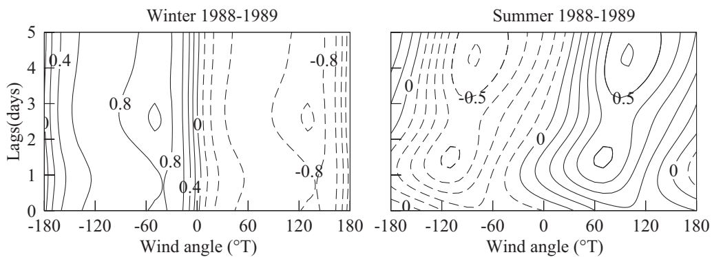
Figure 11. Correlations between observed subtidal currents at 10 m depth and surface wind velocity at 10 m height for the winter and summer seasons of 1988–1989. Analysis was done by projecting subtidal currents to the northwest direction. The critical value was 0.22 for a 95% confidence level.
