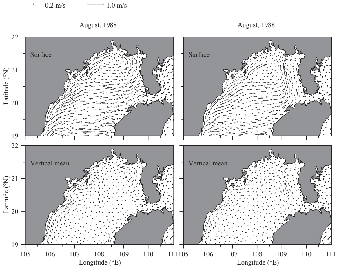
Figure 17. Maps of Global-FVCOM-computed August (top) monthly averaged surface and (bottom) vertically averaged current vectors in the northern Gulf of Tonkin for the stratified cases (left) with only wind forcing and (right) with wind plus tidal forcing.
