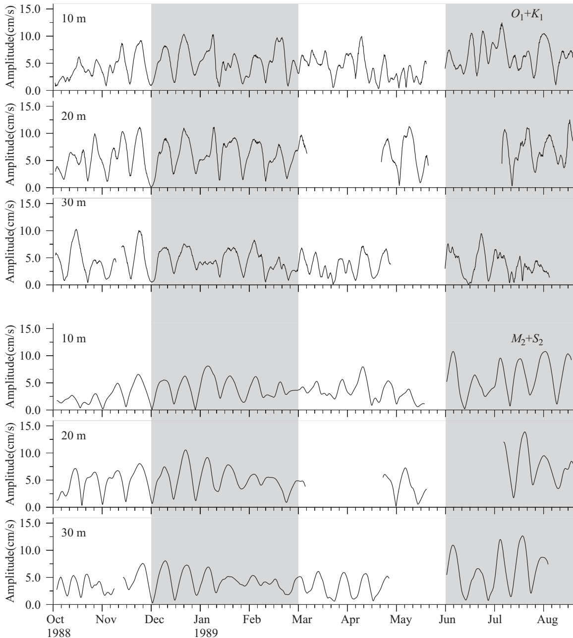
Figure 8. Time series of amplitudes of diurnal and semidiurnal tidal currents calculated using band-passed complex demodulation at depths of 10, 20, and 30 m from October 1988 to August 1989.
