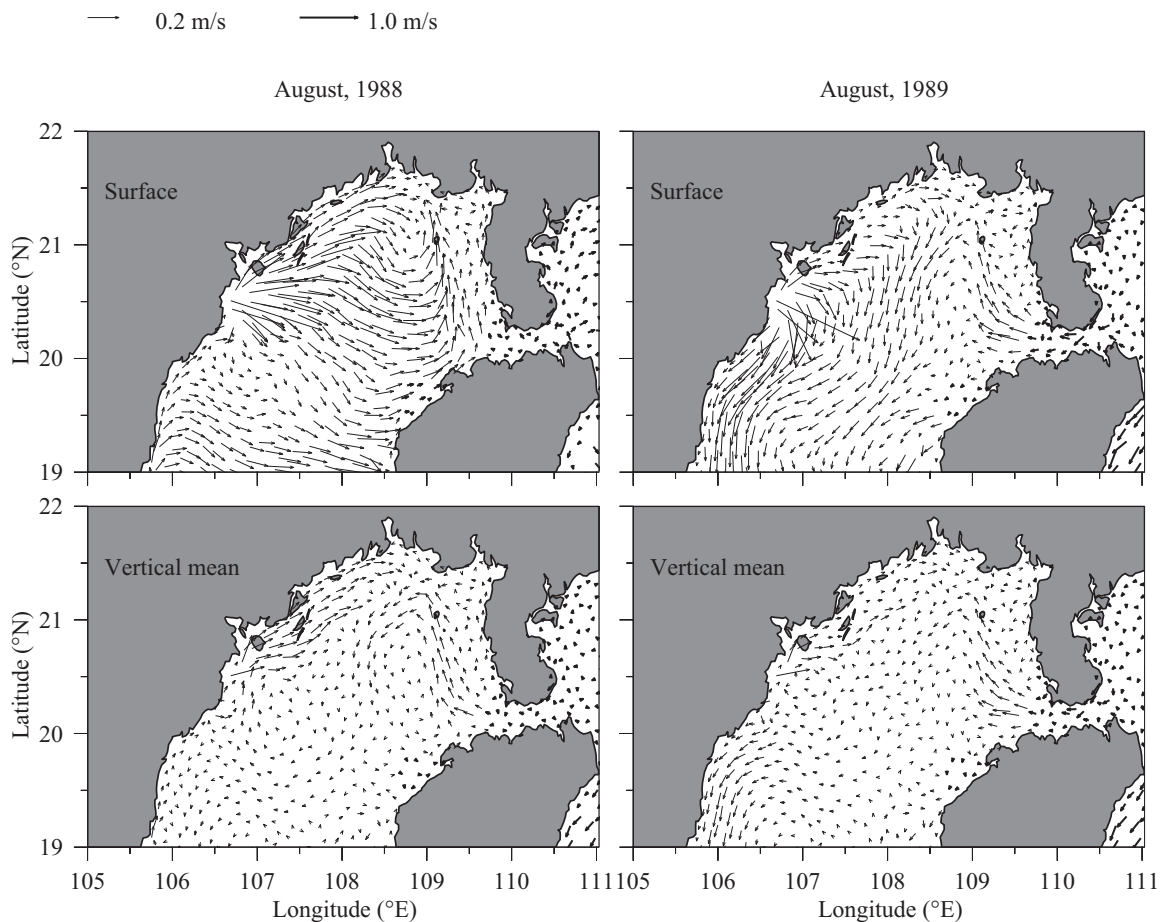
Figure 14. Maps of Global-FVCOM-computed (top) monthly averaged surface and (bottom) vertically averaged current vectors in the northern Gulf of Tonkin for August 1988 and 1989.
