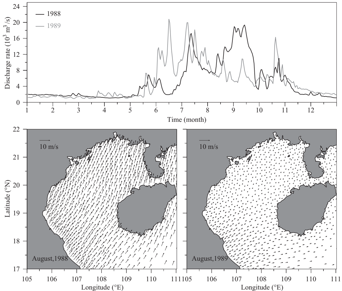
Figure 12. (top) Time series of freshwater discharge from the Hong River over 1988 and 1989, respectively, and (bottom) maps of the monthly averaged 10 m wind velocity for August of 1988 and 1989.
