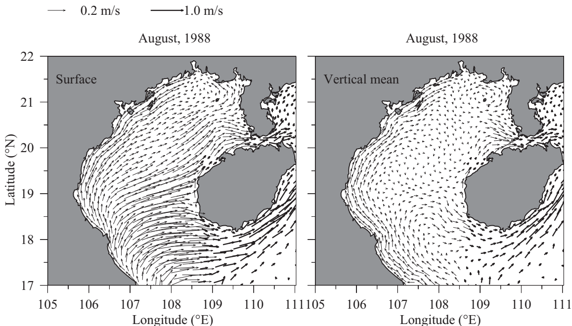
Figure 15. Maps of Global-FVCOM-computed August (left) monthly averaged surface and (right) vertically averaged) current vectors in the Gulf of Tonkin for the homogenous case with only wind forcing (Ex1).
