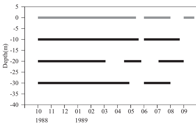
Figure 5. Time line of the 1988–1989 measurements at site A. Black heavy lines: water current measurements. Gray heavy line: wind measurements.
