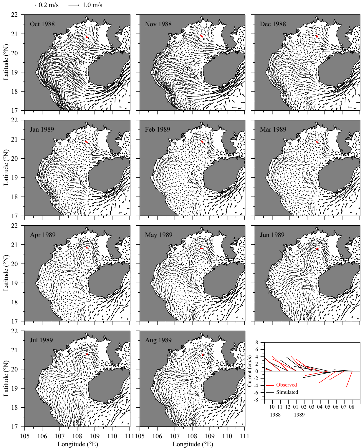
Figure 13. Maps of Global-FVCOM-computed monthly averaged current vectors at 10 m depth in the Gulf of Tonkin for the period October 1988 to August 1989. Monthly averaged current vectors observed at 10 m depth at site A are superposed in these figures (red vectors). The comparison of the 10 m model-computed and observed monthly mean vector currents at site A is shown in the bottom right plot.
