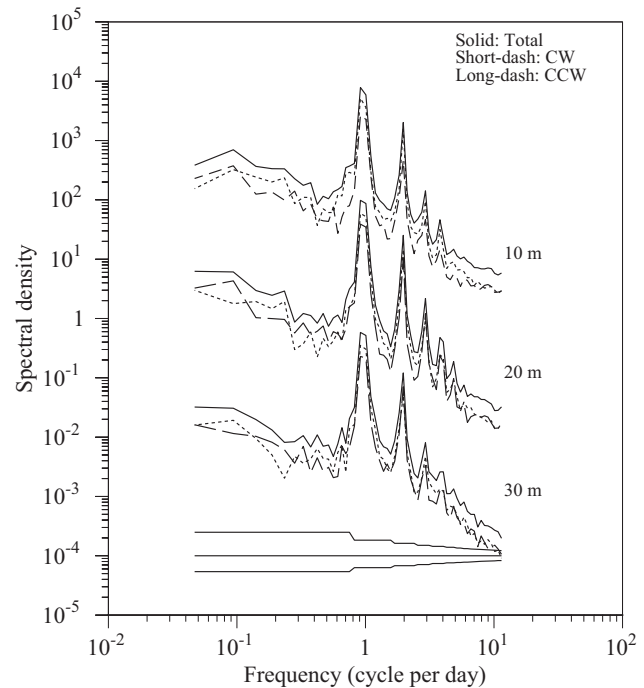
Figure 6. Rotary spectra of water velocities measured at depths of 10, 20, and 30 m during the 1988–1989 deployment. Total: the total energy. CW: the clockwise energy. CCW: the counterclockwise energy. The spectra at the depth of 20 m are shifted downward by 10^2 , and spectra at the depth of 30 m are shifted downward by 10^4 . Rotary spectra were estimated using the hourly data. Spectra density is in (\text{cm/s})^2/\text{cpd} .
