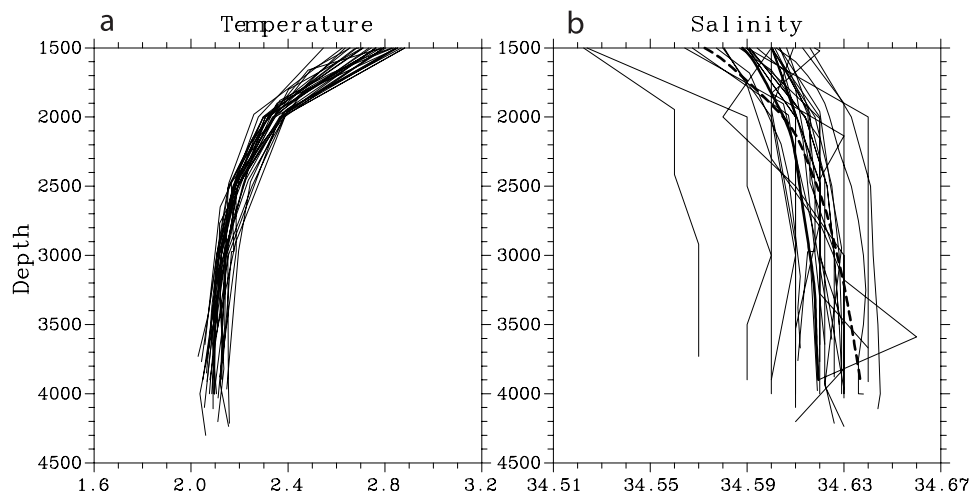
Figure 4. Vertical profiles of potential temperature (°C) and salinity (psu) of those (33) extending to 3500 m or below in the deep South China Sea. The thick solid line on Figure 4b represents the simply averaged salinity, and the thick dashed line represents the synthetic salinity from the 33 profiles.
