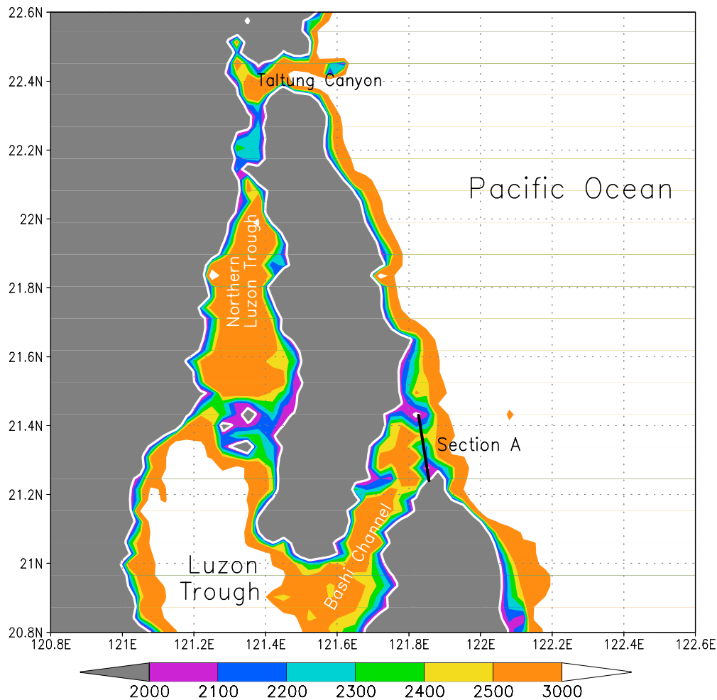
Figure 8. Bottom topography in the Luzon Strait [Smith and Sandwell, 1997].
