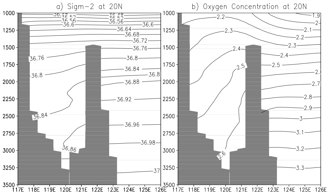
Figure 6. Potential density, \sigma_2 , in \text{kg m}^{-3} and oxygen concentration in \text{mL L}^{-1} at 20^\circ\text{N} . Shading corresponds to bottom topography on the 0.5^\circ grid, and so does not indicate the deepest passages through Luzon Strait.
