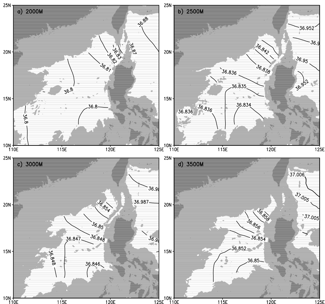
Figure 5. Potential density, \sigma_2 , in \text{kg m}^{-3} calculated from the synthetic salinity in the deep South China Sea.
