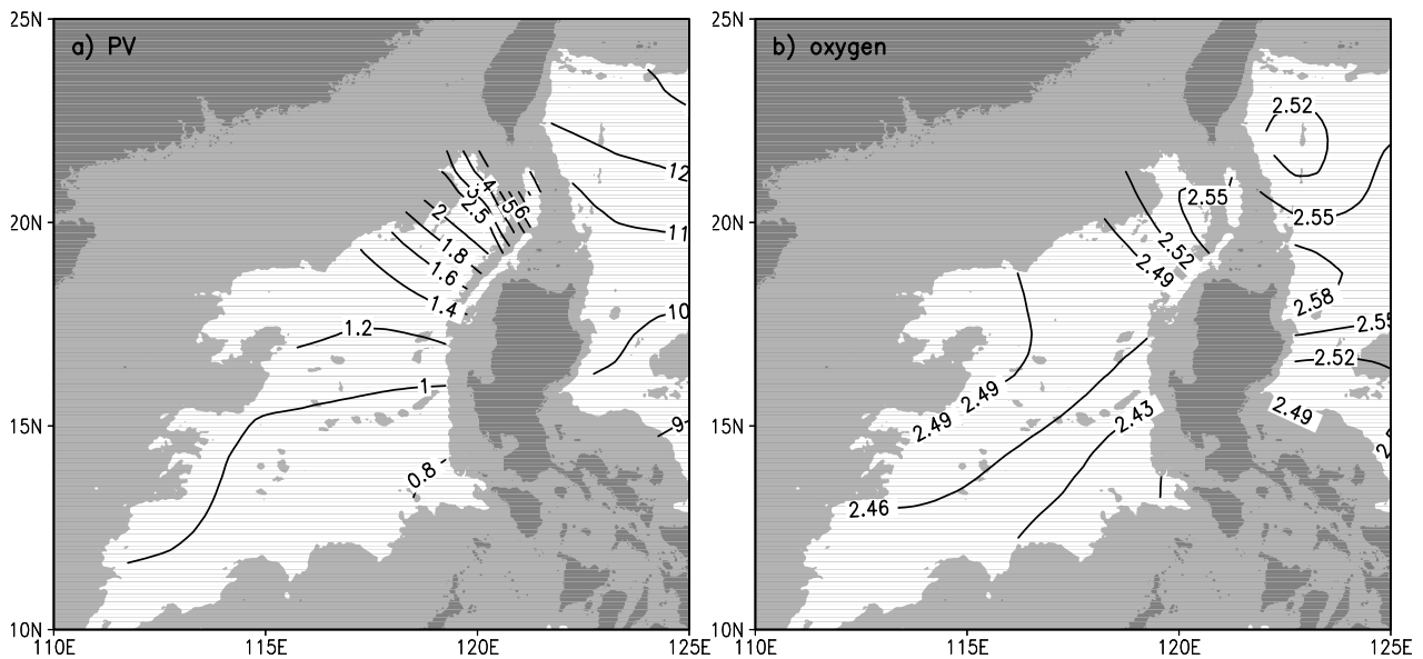
Figure 10. (a) Potential vorticity, defined as \rho_0^{-1} f \partial\rho/\partial z ( 10^{-12} \text{ m}^{-1} \text{ s}^{-1} ), and (b) dissolved oxygen concentration ( \text{mL L}^{-1} ) along \sigma_2 = 36.84 density surface, lying at depths roughly between 2000 and 3000 m in the South China Sea. Here f is the Coriolis parameter, \partial\rho/\partial z is the vertical density gradient, and \rho_0 is a constant reference density ( 10^3 \text{ kg m}^{-3} ).
