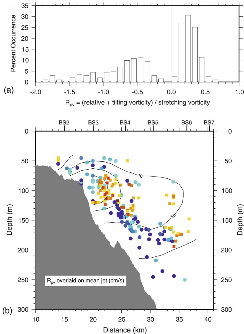
FIG. 7. (a) Histogram of the positive and negative extrema of R_{pv} for the collection of sections. (b) Scatterplot of the extrema of R_{pv} overlaid on the mean along-stream velocity section of Fig. 5.
