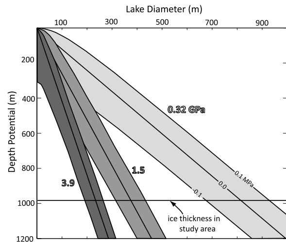
Figure 3. Maximum propagation depth of a water-filled crack versus lake-diameter. Stress and moduli contours are as in Figure 1. Thick black line shows ice thickness of 980 m in the western Greenland study area.
