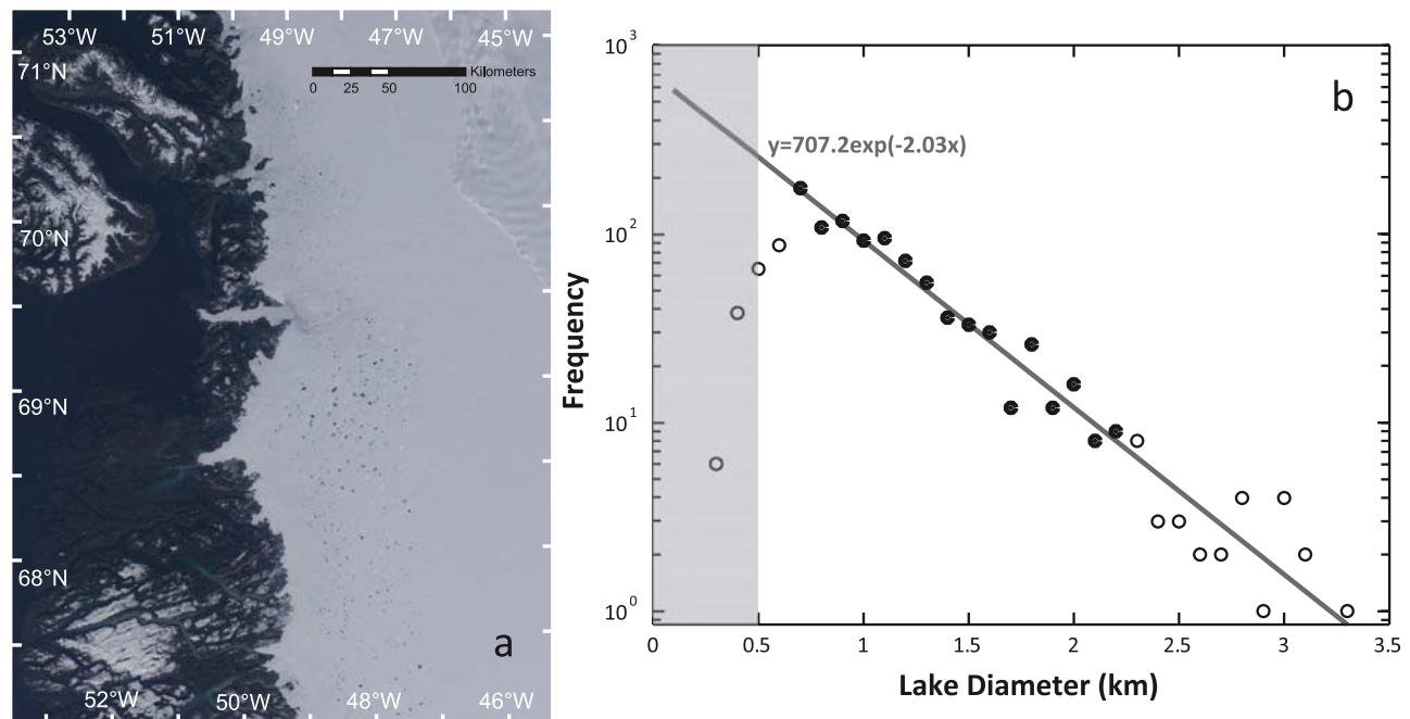
Figure 4. (a) Satellite view of the supraglacial lakes on the West Greenland Ice Sheet near Jakobshaven Isbræ during summer 2006. (b) Supraglacial lake size-frequency distribution binned in increments of 100 m diameter. Filled circles show data that were regressed, open circles show data for lakes that are too small to be reliably counted by the satellite resolution, or too large to be statistically meaningful. The shaded region shows the lakes that are too small to propagate a crack to the ice sheet bed. Based on this distribution, there are >1000 lakes that contain sufficient water to drive hydro-fractures to the ice bed.
