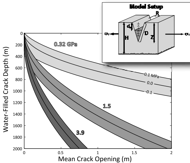
Figure 1. Mean opening width versus depth of a water-filled crack for varying far field stresses. Mean openings are shown for 3 different shear moduli of ice (0.32, 1.5, and 3.9 GPa illustrated in darkening shades of grey). Each field is centered on the curve for a neutral stress regime, and shows the range of differential stresses from -0.1 MPa (compression) to 0.1 MPa (tension). Calculations assume a 100% water filled crack. Figure inset shows the variables and geometry considered for our model.
