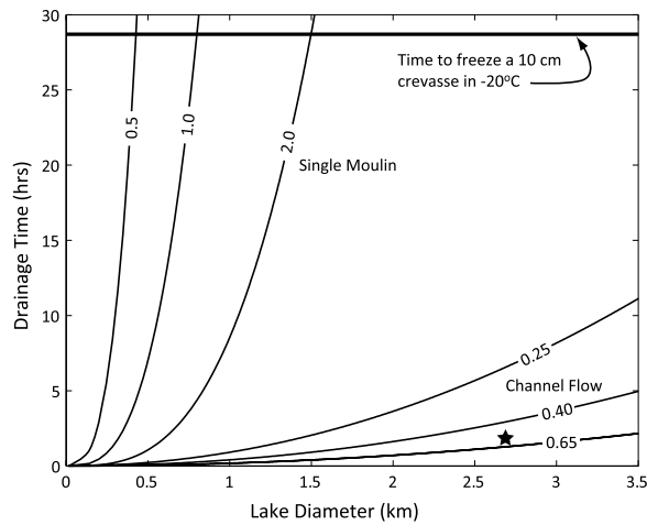
Figure 2. End member drainage times are calculated assuming pipe (moulin) and channel (crack) flow. Pipe flow curves are labeled with conduit diameter, and the channel flow curves are labeled by opening width (in meters). The time to refreeze a 10 cm crevasse is also shown (thick black line [Alley et al. , 2005]). All calculations assume zero differential stress. Star illustrates the drainage time of a 2.7 km diameter supraglacial lake observed by Das et al. [2008].
