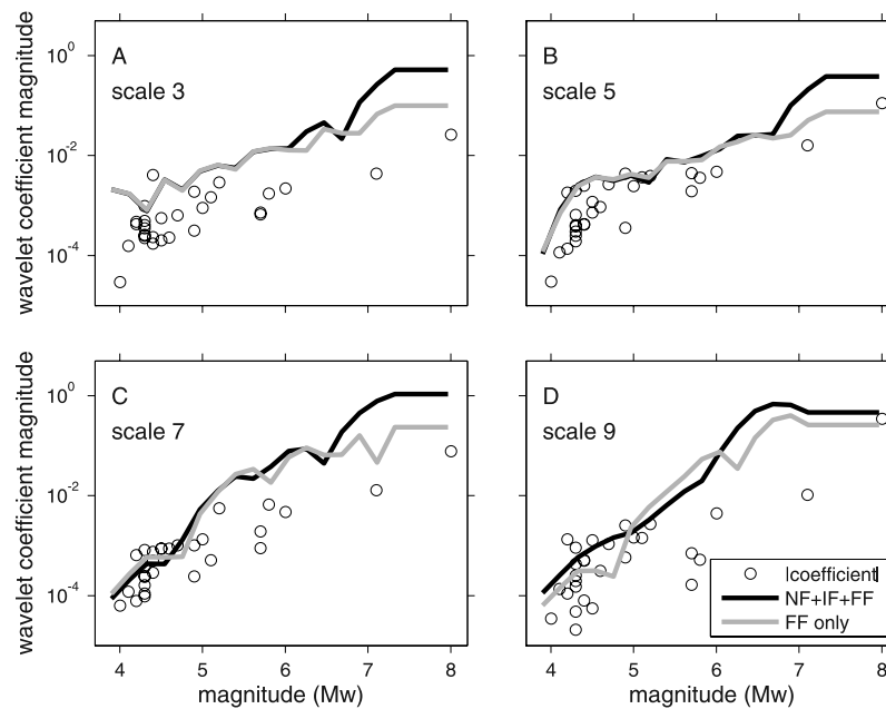
Figure 3. Comparison of peak amplitude of the wavelet coefficients at scales (a) 3, (b) 5, (c) 7, and (d) 9 (white circles) with the earthquake M_w estimate. The gray and black lines denote the coefficient values resulting from a wavelet transform of the velocity seismograms expected for the Sato and Hirasawa (SH) source model for a stress drop of 10 MPa. At this large stress drop, there is a difference in the first 4 s of the seismogram between M_w 7.1 and M_w 8.1, at values of stress drop below 5 MPa there would be no difference in the wavelet coefficients above M_w 7. The black lines include near and intermediate-field terms [Aki and Richards, 2002, equation (4.32)], while the gray line includes only the far-field term. The SH model used a P -wave velocity of 6 km/s, a rupture velocity of 2.5 km/s, an epicentral distance of 20 km, and a shear modulus of 3 \times 10^9 , and a ray takeoff angle \theta = 60^\circ . To scale for propagation effects, the SH curves have been pinned to the median value of the observed coefficient magnitudes at M_w 4.3.
