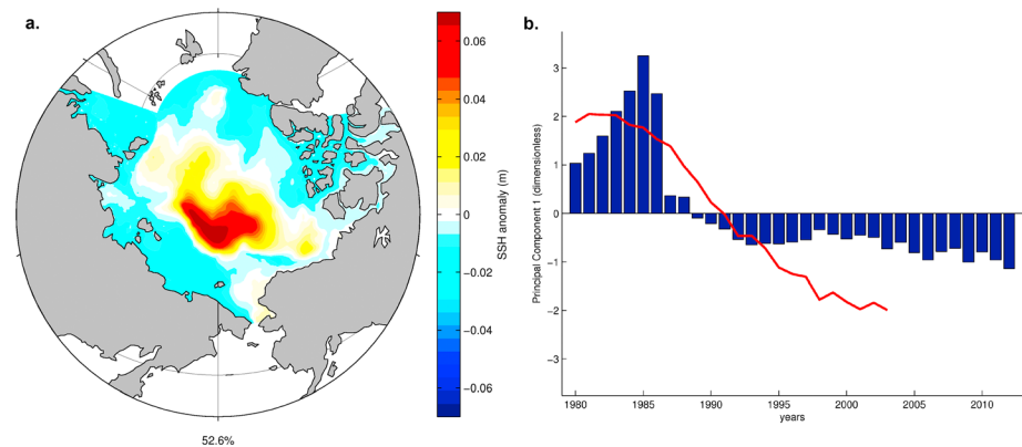
Figure 5. First mode of EOF analysis of sea surface height across the Arctic Ocean. This mode describes 52.6% of the variability. A raised area that approximately corresponds to the “waiting room” region identified in section 3.2 is apparent and varies on a time scale that correlates ( r = 0.83 ) with the EOF indices calculated in Figure 3. The indices from Figure 3b (from 1980 to 2003) are replotted as a red line in Figure 5b.
