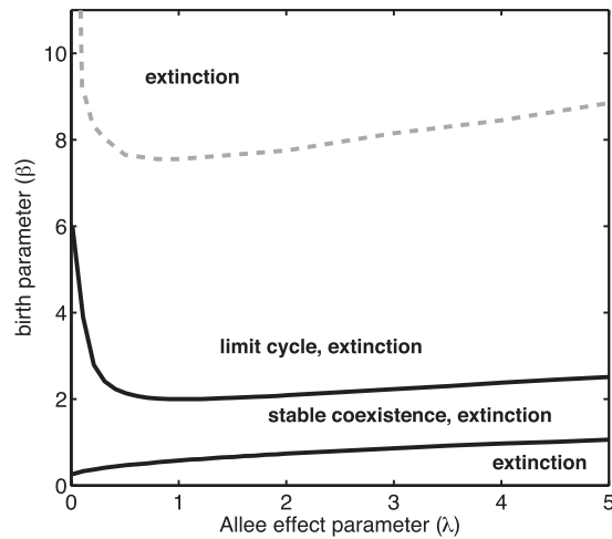
Figure 1-9: Dynamical regimes of the model for different values of the Allee effect parameter ( \lambda ) and the birth parameter ( \beta ). Solid black lines bound the region of stability of the coexistence equilibrium. Lower curve indicates a saddle-node bifurcation; below it, extinction of the predator is the only attractor. Higher black curve indicates a super-critical Hopf bifurcation; above it, the coexistence equilibrium exists but is unstable. The dashed gray line represents a homoclinic bifurcation, and delimitates the region of existence of a stable limit cycle; the curve is drawn based on results from numerical experiments. Parameters are \chi = 0.8 , \delta = 0.1 .
