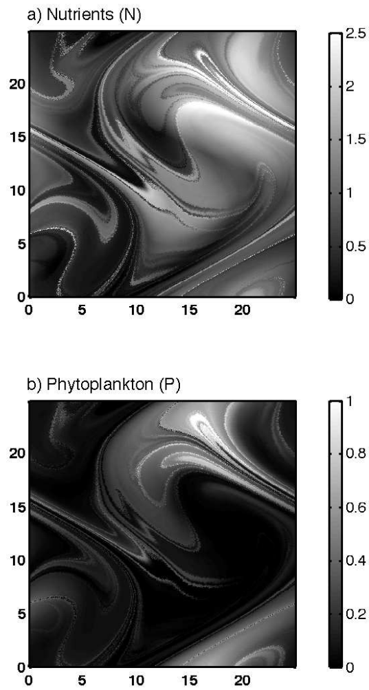
Figure 4-8: Snapshots from simulations with turbulent advection. a) nutrient concentration; b) phytoplankton density. Lighter shades of gray indicate larger values. The two fields tend to be anti-correlated.
