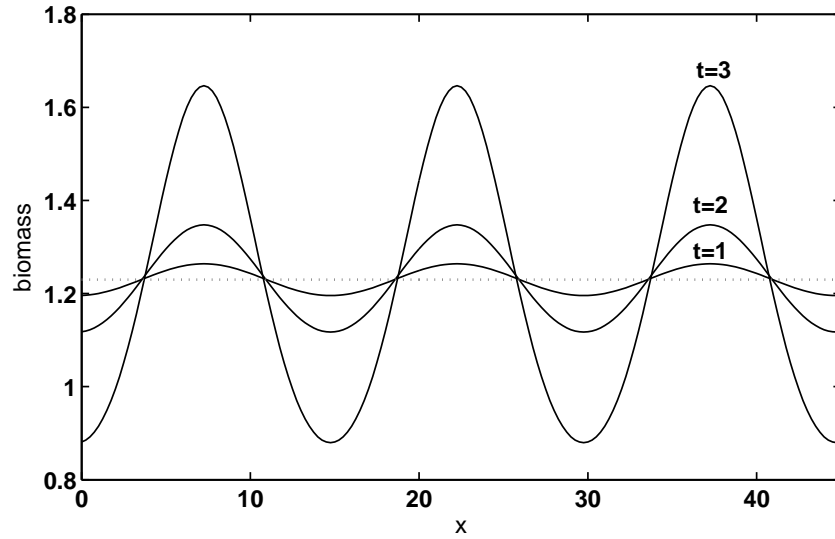
Figure 3-1: Initial growth of patches in the predator distribution. Parameters are S = 2 , \nu = 10 , \gamma = \lambda = 1 , \chi = 0.5 , \delta = 0.1 ; the weighting function is W = e^{-x^2/2} - 1.2e^{-x^2} . The scale of patchiness is determined by the mode with the largest growth rate. Dotted line indicates mean biomass.
