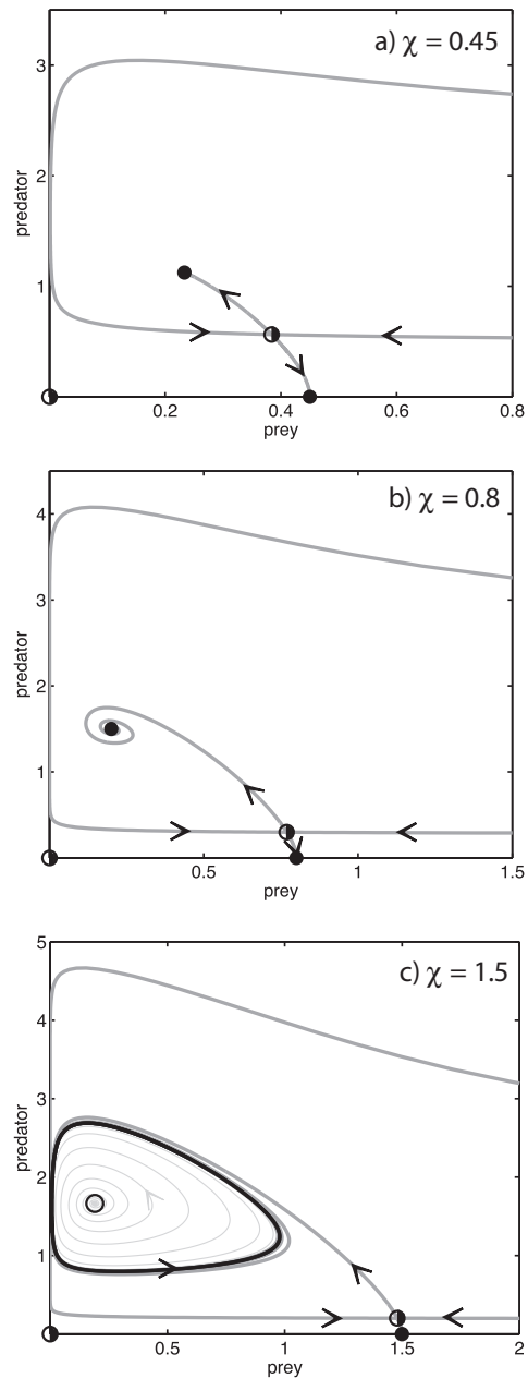
Figure 1-7: Basin of attraction for the coexistence equilibrium, for different values of the enrichment parameter; from top to bottom: \chi = 0.45 , \chi = 0.8 , \chi = 1.5 . Thick lines show the saddle's manifolds; black dots indicate attractors; half-filled circles, saddle points; an empty circle, a repeller. Thin line in bottom plot shows a trajectory with initial condition near the unstable equilibrium, being attracted to the limit cycle. All initial conditions within the area delimited by the stable manifold lead to coexistence. Other parameters are \beta = \lambda = 1 , \delta = 0.1 .
