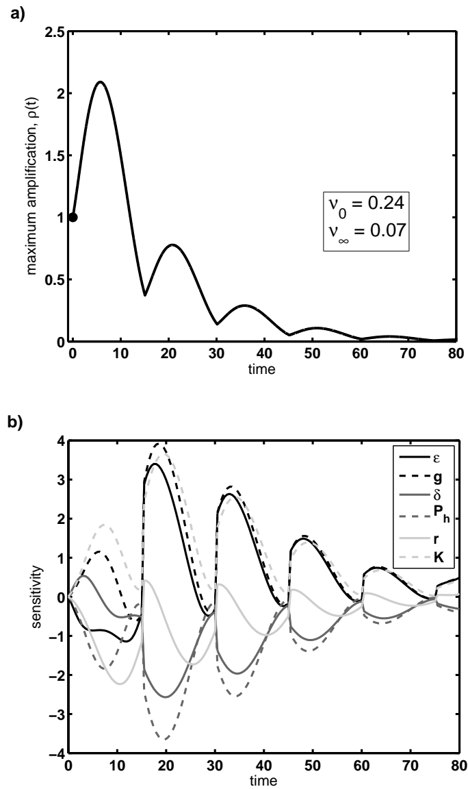
Figure 5-2: a) The amplification envelope \rho(t) for Equilibrium A of the predator-prey model (5.54–5.55), showing the potential amplification of random perturbations. Maximum growth occurs at t = 5.7 . b) The sensitivity of the amplification envelope to the log of each parameter, as a function of time.
