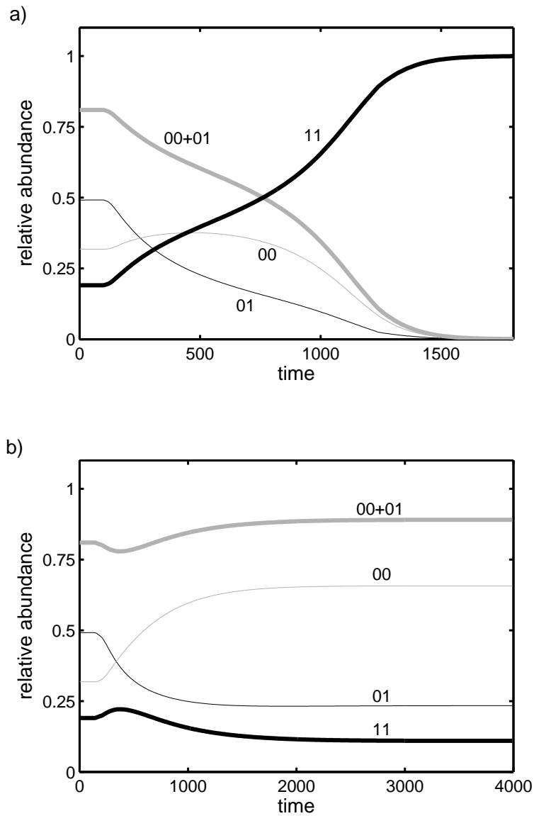
Figure 2-8: Frequency of zooplankton types versus time, for two different values of the parameter \tau , with \mathcal{S} = 5 . a) \tau = 0.04 , the grouping type (11, thick black curve) outcompetes the resident population (00+01, thick gray curve). b) \tau = 0.1 , the grouping type aggregates but does not invade the resident population. Decreasing \tau has the effect of accelerating mixing relative to predation, thus effectively increasing resource supply to clustered zooplankton. Initially the grouping type represents a fraction f_c of the population.
