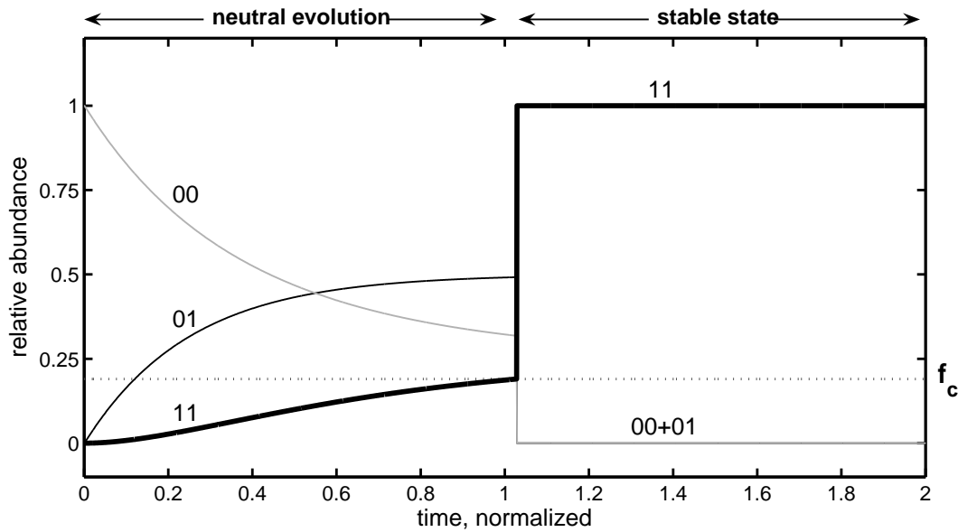
Figure 2-7: Frequency of zooplankton genotypes versus time, showing invasion of a non-grouping population by the grouping type; S = 5 , \tau = 0.04 ; V = 0 . Dotted line indicates the critical frequency f_c ; other curves show the relative abundance of types 00 (thin gray), 01 (thin black), and 11 (thick black). Time is normalized by the mutation timescale, \delta^{-1} . The new allele, introduced at low frequency at t = 0 , does not affect fitness until the frequency of grouping organisms (type 11) reaches f_c , at which point it starts to aggregate. Abrupt changes in allele frequencies at t \approx 1 result from ecological dynamics, which occur rapidly compared to the mutation timescale; details are shown in Figure 2-8. In this case, social behavior is a successful strategy: the grouping type wins the competition and the other types become extinct. The ecosystem is then stable with respect to mutations in the two-allele model.
