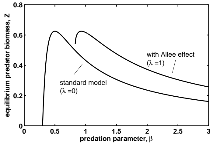
Figure 1-12: Equilibrium predator biomass Z^* (dimensional units) vs grazing parameter. Only real positive coexistence equilibrium is shown (for \lambda = 1 , the equilibrium corresponding to higher predator density is plotted). Parameters: \epsilon = 0.5 , P_h = 1 , \delta = 0.1 , \chi = 0.5 .
