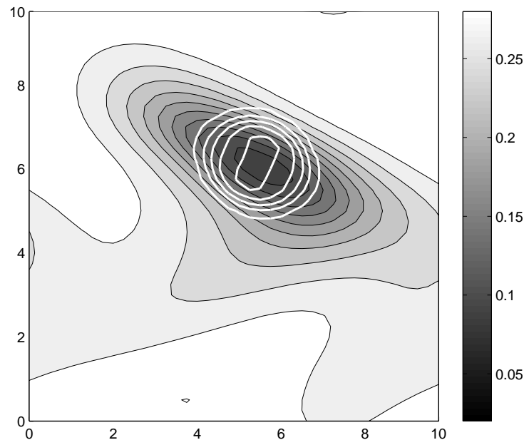
Figure 2-9: Contours of zooplankton biomass, white lines, superimposed on the phytoplankton field, gray shades. This shows stirring of resources by the turbulent field, for parameters \mathcal{S} = 5 , \tau = 0.1 , and V = 5 .
