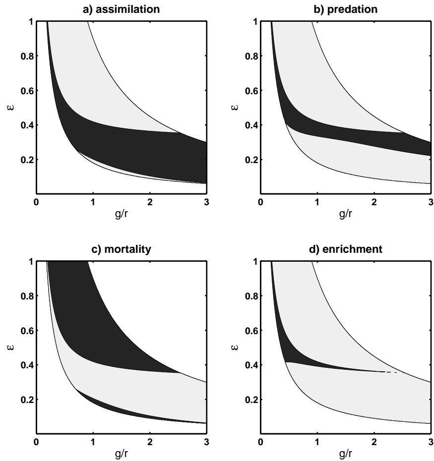
Figure 5-5: The sign of the sensitivity of reactivity of the predator-prey model (5.54–5.55) in the region of parameter space where the coexistence equilibrium is stable. Dark areas indicate negative sensitivity to the non-dimensional parameters, light gray areas indicate positive sensitivity. Sensitivity of \nu_0 to a) assimilation ( \epsilon ), b) predation ( g/r ), c) mortality ( d/r ), and d) enrichment ( K/P_h ).
