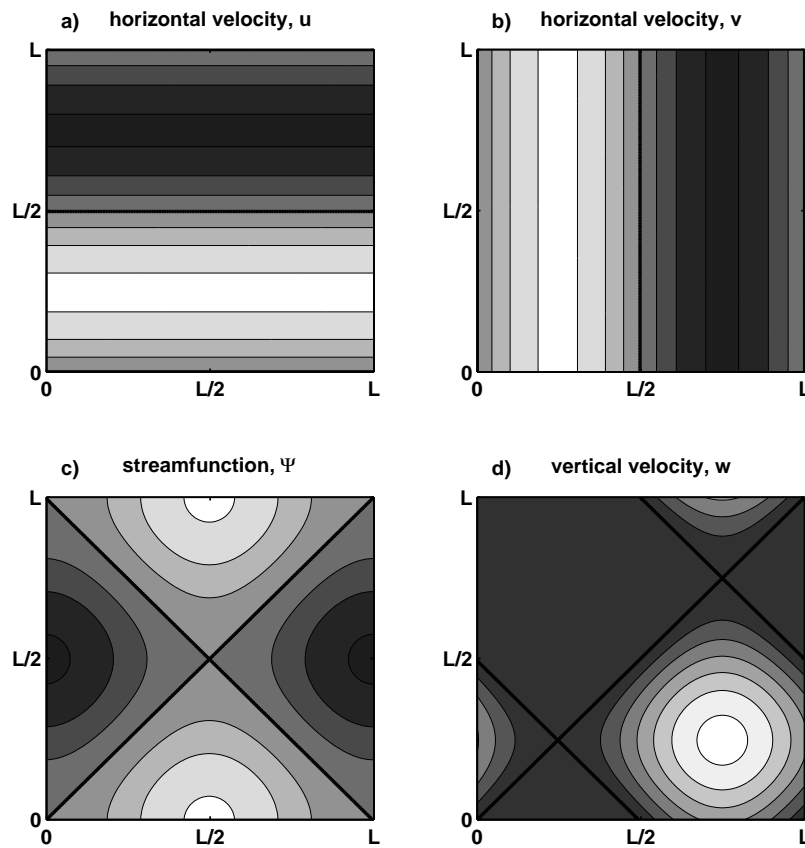
Figure 4-7: Circulation patterns in the turbulent map. a,b) Horizontal velocity. c) Streamfunction. d) Vertical velocity. In this specific example, the instantaneous phases vanish, \phi_u = \phi_v = 0 , and are evolving at the same rate, \frac{d\phi_u}{dt} = \frac{d\phi_v}{dt} > 0 . Values increase from black to white; thick black curves indicate the zero contour.
