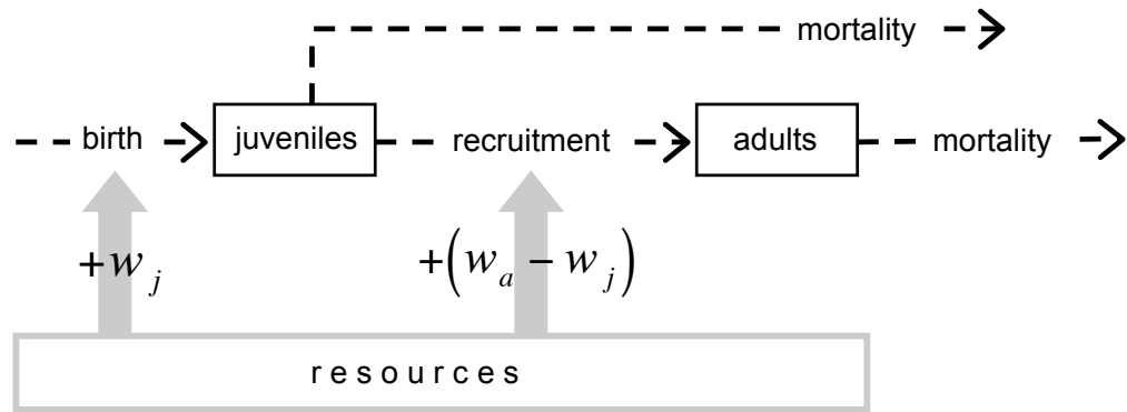
Figure 1-1: Life cycle of the 2-stage predator population. Juveniles and adults have an average weight of w_j and w_a , respectively. Generation of new biomass through birth and recruitment is taken out of the resource.
