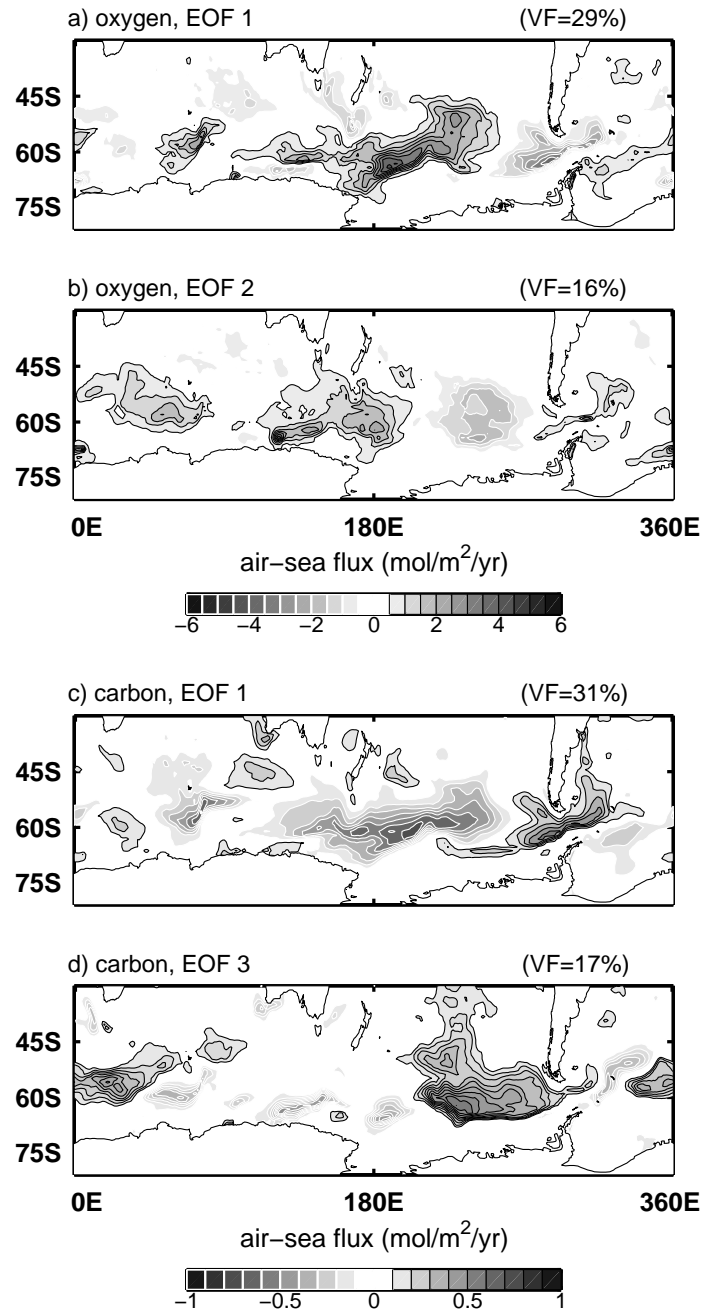
Figure 6-4: Spatial patterns of the leading empirical orthogonal functions, for air-sea flux variability of oxygen (a, b) and carbon dioxide (c, d), and fraction of the total variance (VF) associated with each mode. Black (white) contours denote positive (negative) fluxes into the ocean. SAM is associated with the first EOF of O 2 and CO 2 fluxes; ENSO is associated with the second EOF of O 2 fluxes and the third EOF of CO 2 fluxes. The second EOF of CO 2 fluxes, not shown, is not correlated with SAM or ENSO.
