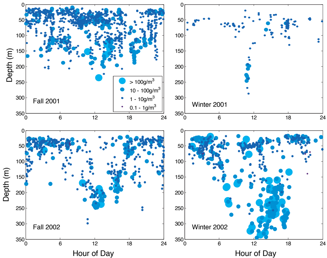
Figure 4-10: Observed aggregations of Antarctic krill from acoustic measurements. Each dot represents an aggregation, plotted as a function of the time of day when it was observed (x-axis) and its mean depth (y-axis). Size and color of dots indicate the mean density of aggregations (see legend). [Figure courtesy of Gareth Lawson; adapted from Lawson (2006).]
