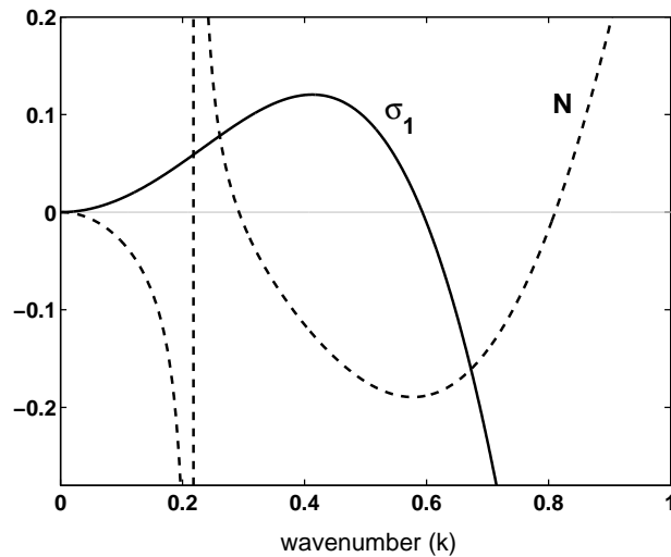
Figure 3-2: Linear growth rate (solid) and nonlinear coefficient (dashed). Population dynamics terms are neglected ( \nu \rightarrow \infty ); other parameters as in Figure 3-1. Nonlinearities are stabilizing in the wavenumber region where \sigma_1 > 0 and N < 0 .
