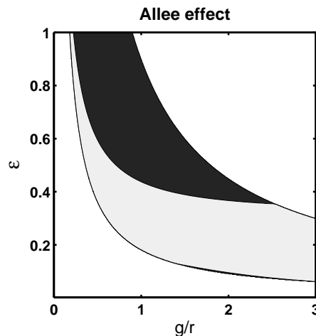
Figure 5-7: Sensitivity of reactivity to the Allee effect parameter c ; light gray (dark gray) areas indicate positive (negative) sensitivity.
