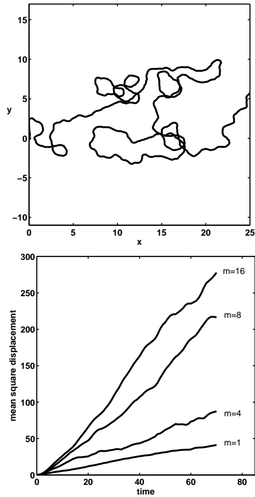
Figure 4-4: Left: Trajectory of a 16-member school initially located at (0, 0) . Right: mean squared displacement of versus time, for different group sizes; m is the number of individuals in a group. Schools disperse faster than random walkers (lower curve, m = 1 ).
