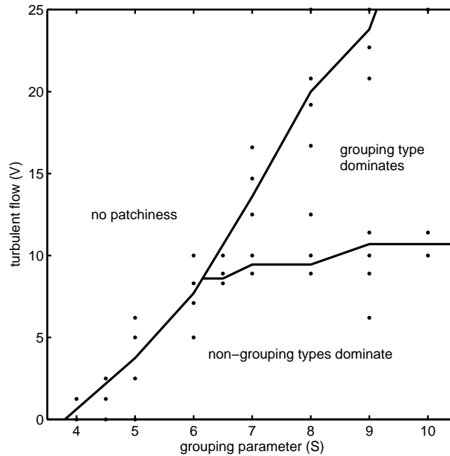
Figure 2-10: Outcome of the competition between grouping and non-grouping types, when the mutant allele is introduced at low density in a resident population of non-grouping organisms. The grouping parameter and strength of turbulent flow are varied; \tau is kept constant ( \tau = 0.1 ). The domain size is D = 10 . Solid lines delimitate three distinct regions of parameter space. Except in the region labeled “no patchiness”, zooplankton with social behavior spontaneously assemble in dense groups. Without turbulent advection ( V = 0 ), they are outcompeted by the non-grouping types and remain a small fraction of the population. Weak flows do not affect the outcome of the competition, but under more turbulent flows the grouping type becomes a better competitor and replaces the non-grouping resident organisms. Black dots indicate parameter values for which numerical simulations were performed.
