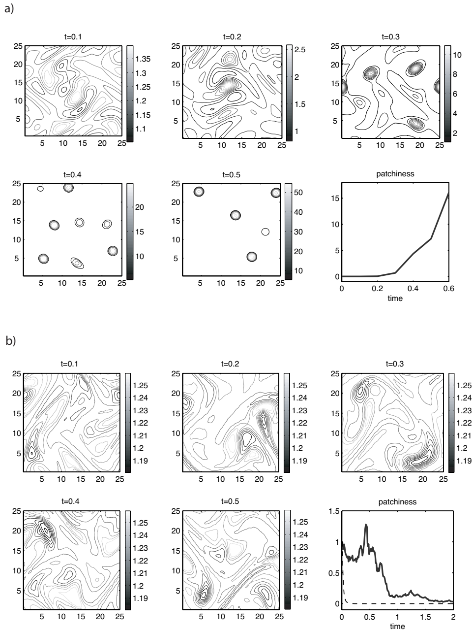
Figure 2-6: Effect of turbulent advection on the development of patches in a population of zooplankton with social behavior, \mathcal{S} = 5 . a) weak flow, V = 2.5 : groups form and merge. The last panel shows an index for patchiness as defined in (2.15), increasing in time. b) strong flow, V = 150 : horizontal shear prevents the development of patches. Stirring and mixing homogenize the zooplankton distribution, which remains spatially more intermittent than a passive scalar field. The last panel shows the index for patchiness normalized by the value at t = 0 ; solid curve is for zooplankton with social behavior, dashed curve is for a passive tracer.
