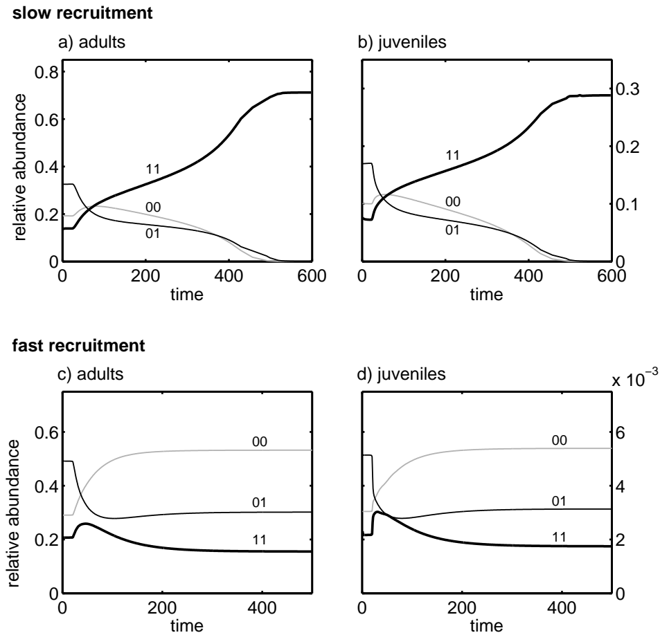
Figure 2-11: Relative abundance of zooplankton versus time in the structured model, for slow recruitment (top) and fast recruitment (bottom). a) and b) q = 1 : the grouping type (11, thick black curve) outcompetes the resident population (00+01, thin curves); the frequency of the grouping allele increases monotonically in the juvenile and adult populations. c) and d) q = 100 : the grouping type does not invade the resident population. When recruitment is fast, juveniles are a negligible fraction of the total population so that the model is equivalent to an unstructured predator-prey model.
