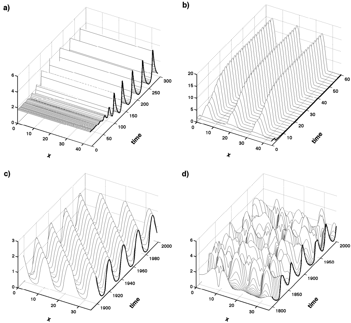
Figure 3-6: Predator biomass in time and space. Thin black contours show the instantaneous spatial distribution, at fixed intervals in time. Thick black curve shows the time series of biomass at a fixed location. a) Without aggregation behavior ( S = 0 ), the predator-prey system reaches a limit cycle after a period of transients; the simulation shown here is initialized near the unstable coexistence fixed point. b) With social behavior ( S = 2 ) and fast diffusion ( \nu = 10 ), patches form spontaneously and the system loses its oscillatory behavior. c) With social behavior ( S = 15 ) and slow diffusion ( \nu = 0.05 ), the system supports a regular wave traveling through the domain; transients are not shown. d) With social behavior ( S = 5 ) and slow diffusion ( \nu = 0.02 ), the density field can appear chaotic. Parameters are, for a, b and d: \gamma = \lambda = 1 , \delta = 0.1 , \chi = 2.5 ; for c: \gamma = 2 , \lambda = 0.1 , \delta = 0.2 , \chi = 1 .
