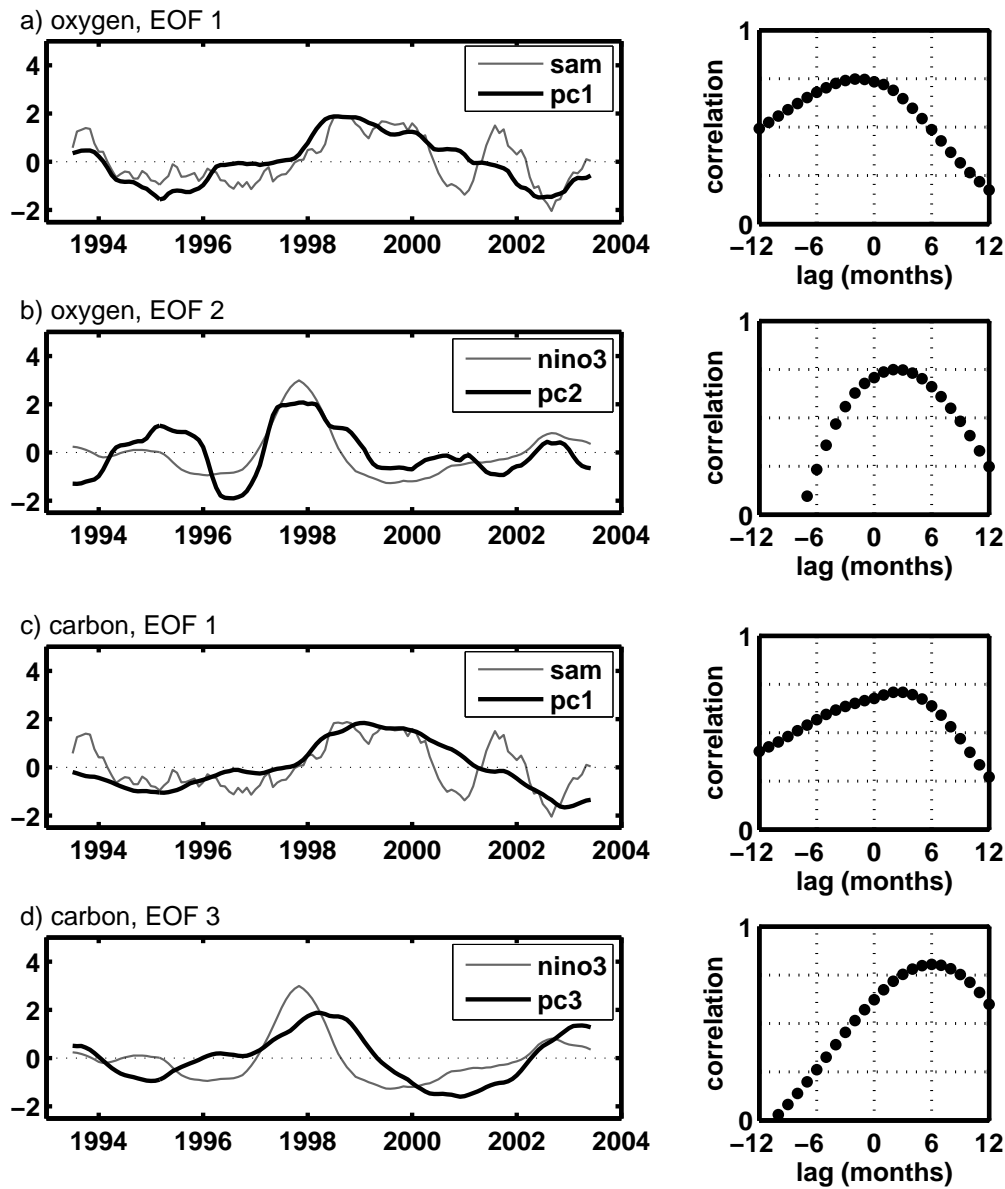
Figure 6-5: Principal components associated with the empirical orthogonal functions of Figure 6-3, along with a) and c) the SAM index; b) and d) the Niño3 index. All time series are filtered with a 12-month running-mean and normalized. Right panels show the lagged correlations between the time series in the left panels; for positive lags, the climate index leads.
