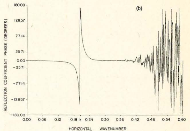
FIG. 13. Magnitude (a) and phase (b) of the computed reflection coefficient for a slow isovelocity fluid bottom.
