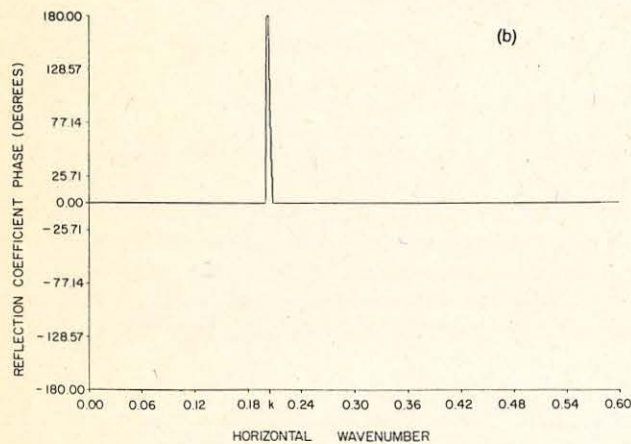
FIG. 12. Magnitude (a) and phase (b) of the exact reflection coefficient for a slow isovelocity fluid bottom.
