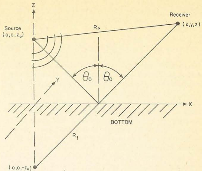
FIG. 3. The direct and specularly reflected arrivals.
