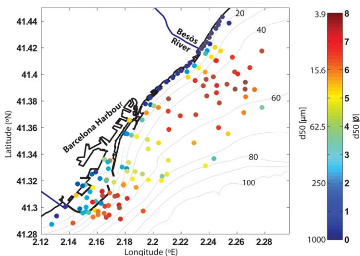
Figure 2. Compilation of historical observations of sediment texture. Grain size expressed in μm and \phi = -\log_2(D_{50}) , where D_{50} is the particle size in mm. The bathymetry is also included in gray. The deepest isobath plotted is 100 m, which represents the shelf break.
