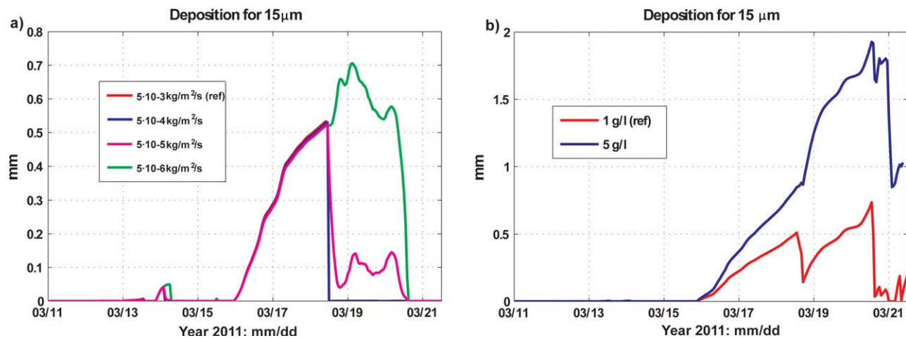
Figure 9. Time series of the deposition rates of the sensitivity tests for the sediment class 15 \mu\text{m} . (a) Deposition rates at 10 m water depth (P1) for different erodibility constant values ( E_0 in \text{kg}\cdot\text{m}^{-2}\cdot\text{s}^{-1} ). Note that the blue line overlaps the red line. (b) Deposition rates at 30 m water depth (30 m) for different suspended sediment river yield: 1 and 5 \text{ mg}\cdot\text{L}^{-1} . The reference simulation is marked in both plots in red. Note that the y axis value varies in both subplots. Dates in x axis represent month/day.
