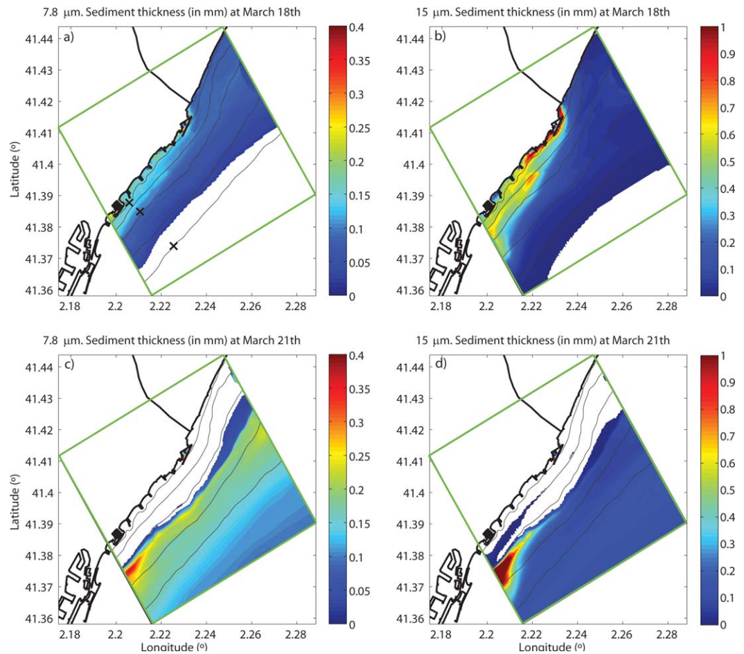
Figure 5. Modeled sediment deposition for (a, b) 18 March at 00:00 and (c, d) 21 March at 00:00 for the LOCAL simulation (the mesh limits are plotted in green) representing both sediment classes: 7.8 and 15 \mu\text{m} . Isobaths are plotted each 10 m. Note that the contour plot varies in ranges. Dark crosses show the control points at 10, 30, and 50 m. When the deposition is zero, the color used is white.
