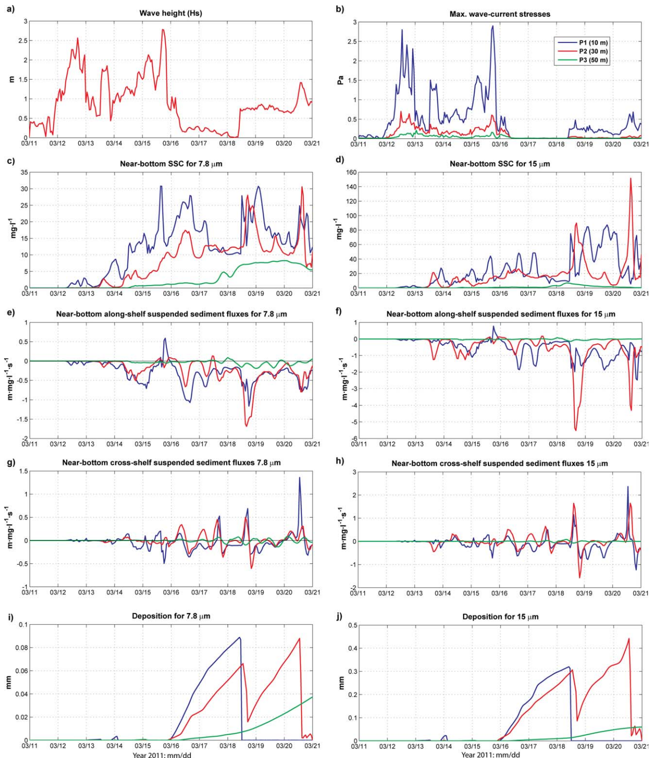
Figure 6. Time series during 11–21 March 2011 at the P1, P2, and P3 control points (see Figure 5a). Left column represents the variables for 7.8 μm sediment class and right column 15 μm sediment class. (a) Significant wave height at P1 (m); (b) combined wave-current bottom stress magnitude (Pa). (c, d) near-bottom Suspended Sediment Concentration (SSC); (e, f) near-bottom along-shelf sediment suspended fluxes; (g, h) near-bottom cross-shelf suspended sediment fluxes; (i, j) deposition thickness. Sediment fluxes are displayed according to the axis directions shown in Figure 1c. Dates in x axis represents month/day.
