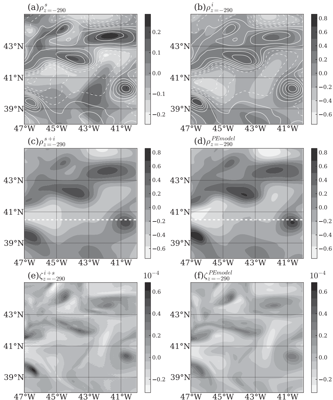
FIG. 7. (a)–(d) The density at 290 m for region 1; (a) \rho^s , (b) \rho^i , (c) \rho^s + \rho^i , and (d) the PE model density. The PE model density in (d) is plotted with white contours in (a), (b) for comparison. The vertical component of the relative vorticity ( s^{-1} ) at 290 m for (e) the total reconstructed field and (f) the PE model are shown. Dashed lines in (c), (d) show the location of the vertical section shown in Fig. 8.
