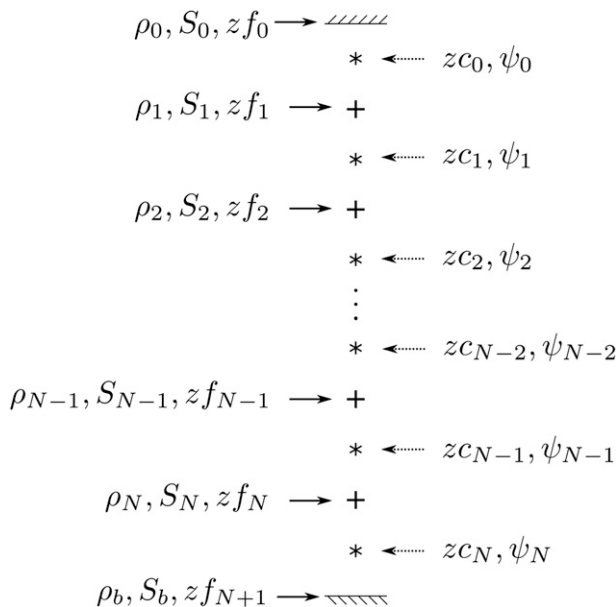
FIG. A1. Variable arrangement in a stagger vertical grid, where S_i = f^2/N^2 at z f_i .
