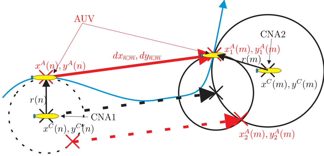
Figure 3-7: Computing two possible positions of the AUV at t(m) ( x_1^A(m), y_1^A(m) and x_2^A(m), y_2^A(m) ) using the dead-reckoning information dx_{n,m}, dy_{n,m} and the information x^C(n), y^C(n) and r(n) received at t(n) from CNA1 and x^C(m), y^C(m) and r(m) received at t(m) from CNA2.
