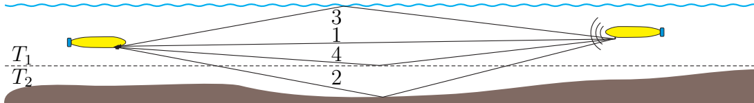
Figure 2-8: Multi-path propagation: in addition to the direct path (1) there are longer paths due to reflection on sea bottom (2), sea surface (3) and a temperature discontinuity (4) (thermocline).
