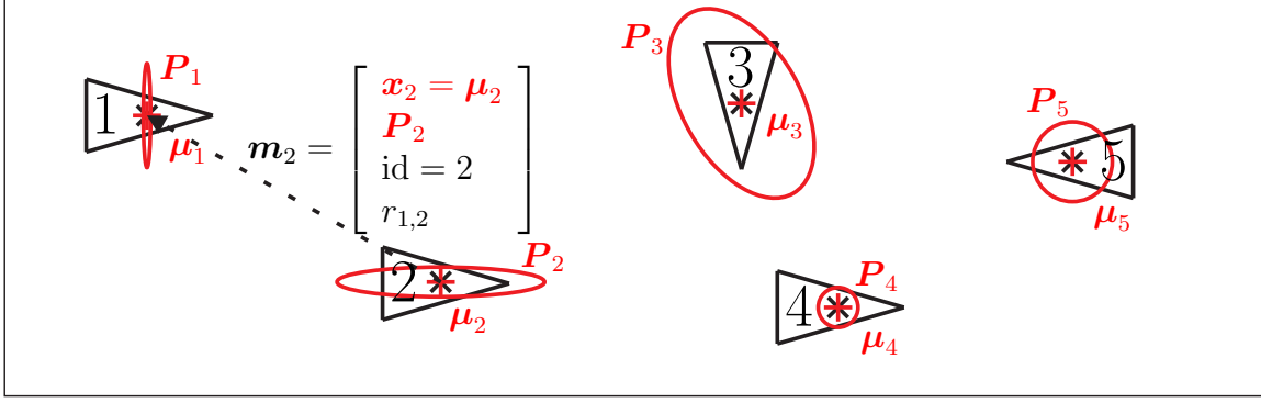
Figure 3-4: A set of 5 vehicles performing CN using an EKF. Each vehicle i maintains the distribution over its state (red) through a mean vector \boldsymbol{\mu}_i and the associated covariance matrix \mathbf{P}_i . This information, along with the unique id is broadcasted to other vehicles.
