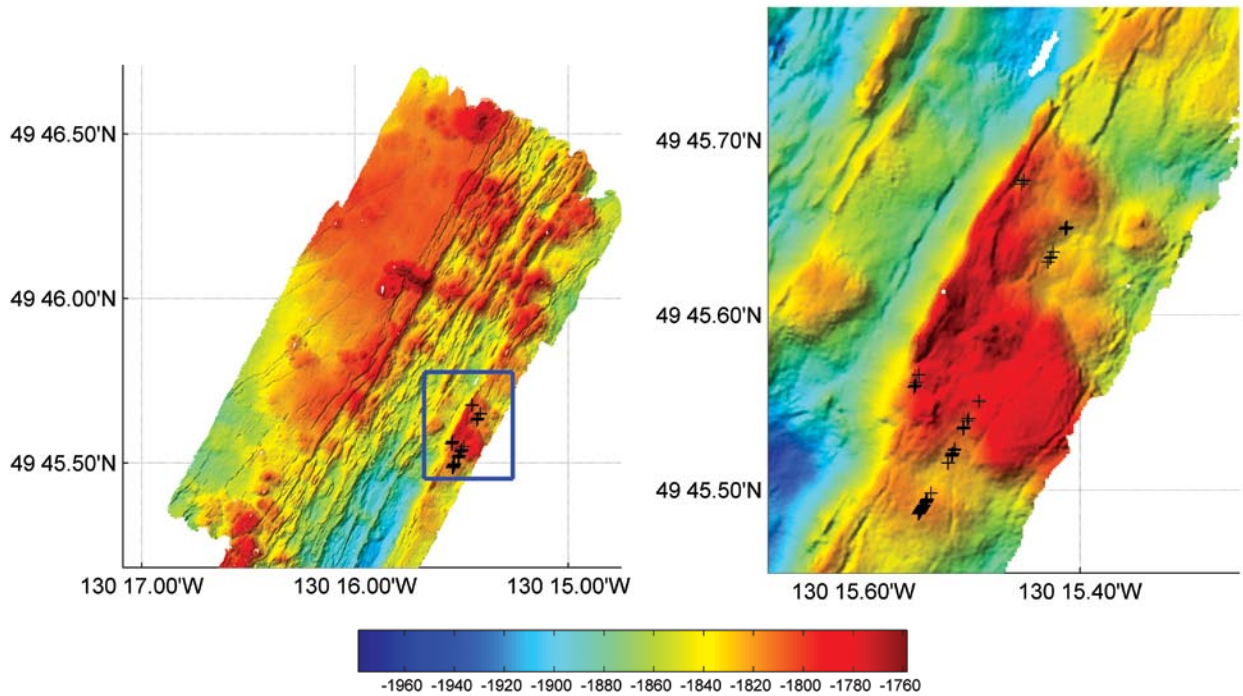
Figure 2. Bathymetry results from the summit of the Southern Explorer Ridge using a multibeam sonar on ABE . The multibeam data permitted quantitative assessment of the faulting of the axial summit graben floor and provided new insights into the formation of the Magic Mountain site, shown in the expanded view. Contradictory to previous reports, the vents were located outside the axial rift graben adjacent to the graben's large eastern bounding fault. The plots also show the location of collocated redox potential signals and temperature anomalies that provided a reliable indication of hydrothermal activity even in complex terrain in the presence of significant currents.
