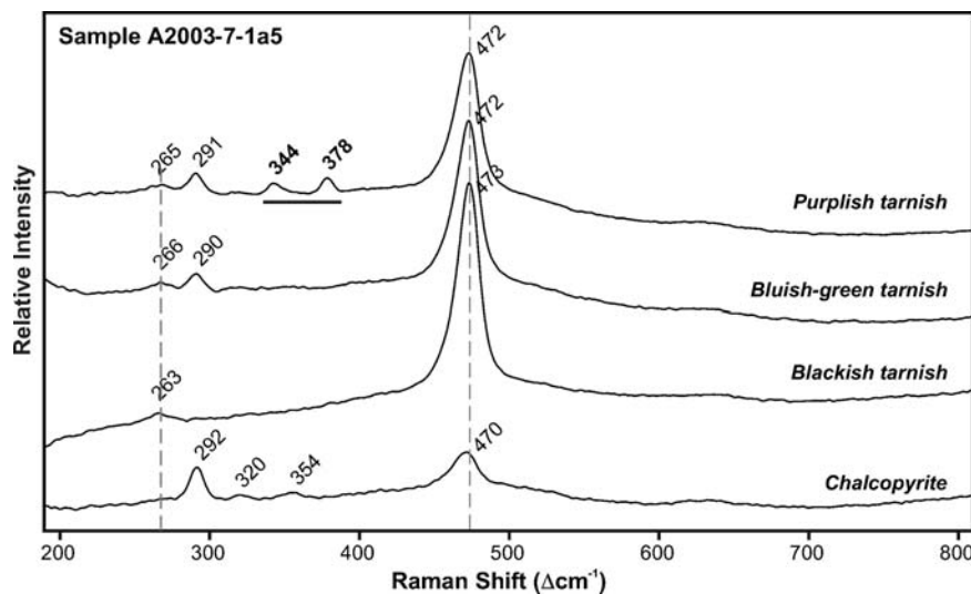
Figure 9. Scan of spectra across the tarnishes on sample A2003-7-1a5 (Figure 5) using the NCO and green excitation. The chalcopyrite spectrum (bottom) was collected from an area on the sample away from the tarnishes. All spectra are 10 x 15 sec exposures.
