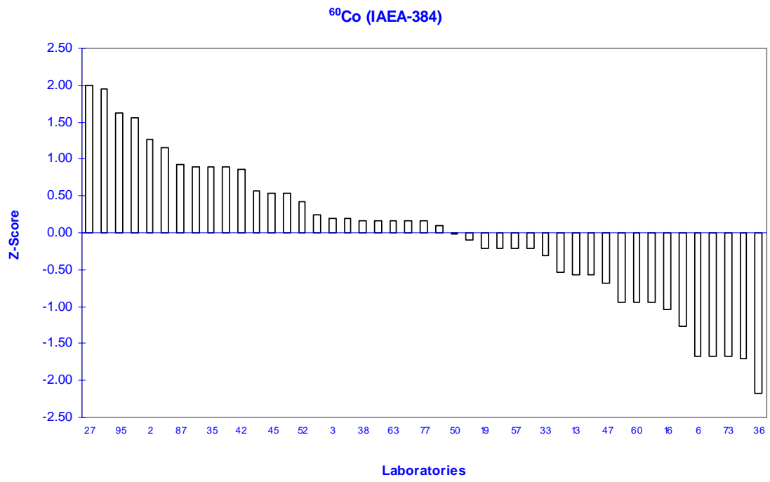
Fig. 1. Z-score values for 60 Co in IAEA-384.
