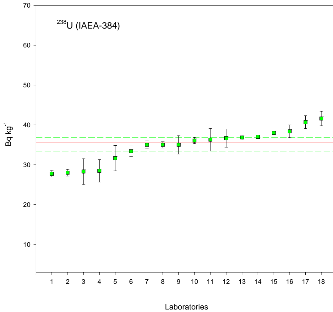
Fig. 5. Data evaluation for ^{238}\text{U} in IAEA-384 (only alpha-spectrometry and mass spectrometry results). The median (solid line) and corresponding 95 % confidence intervals (dashed lines) are also shown.
