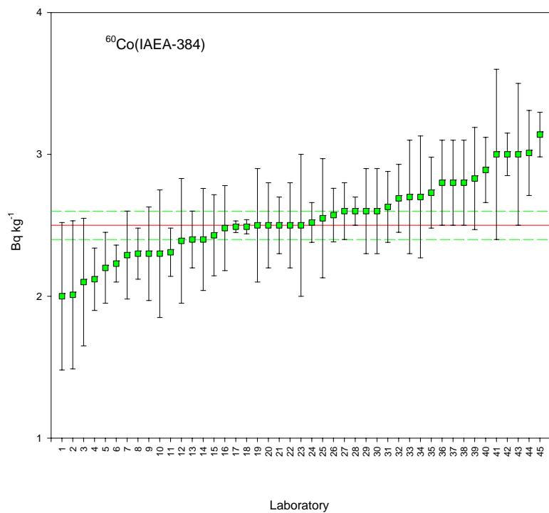
Fig. 2 . Data evaluation for ^{60}\text{Co} in IAEA-384. The median (solid line) and corresponding 95 % confidence intervals (dashed lines) are also shown.
