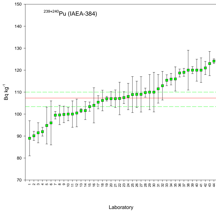
Fig. 3. Data evaluation for ^{239+240}\text{Pu} in IAEA-384. The median (solid line) and corresponding 95 % confidence intervals (dashed lines) are also shown.
