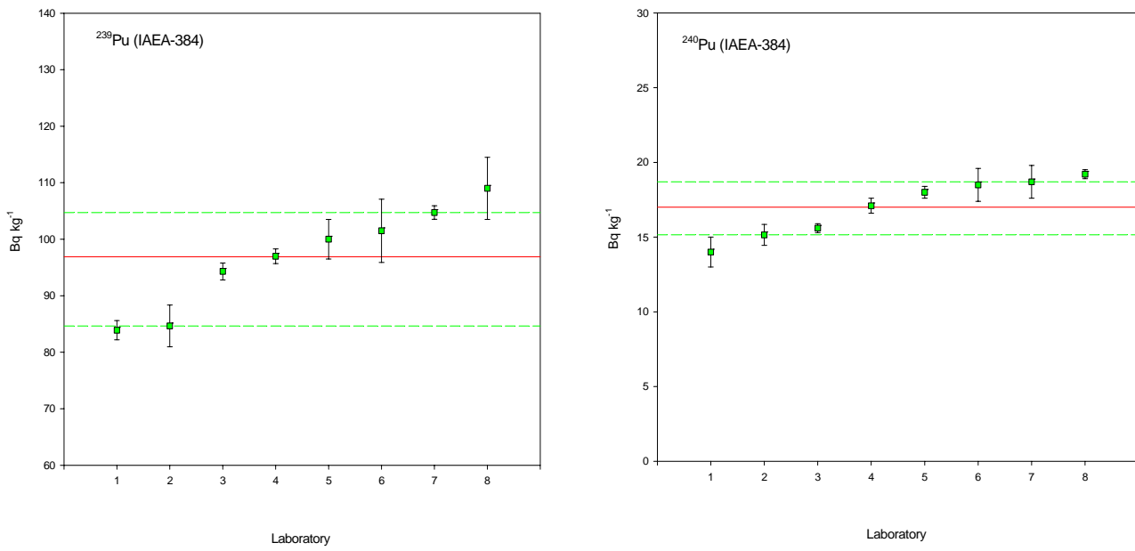
Fig. 6. Data evaluation for ^{239}\text{Pu} and ^{240}\text{Pu} in IAEA-384. The median (solid line) and corresponding 95 % confidence intervals (dashed lines) are also shown.
